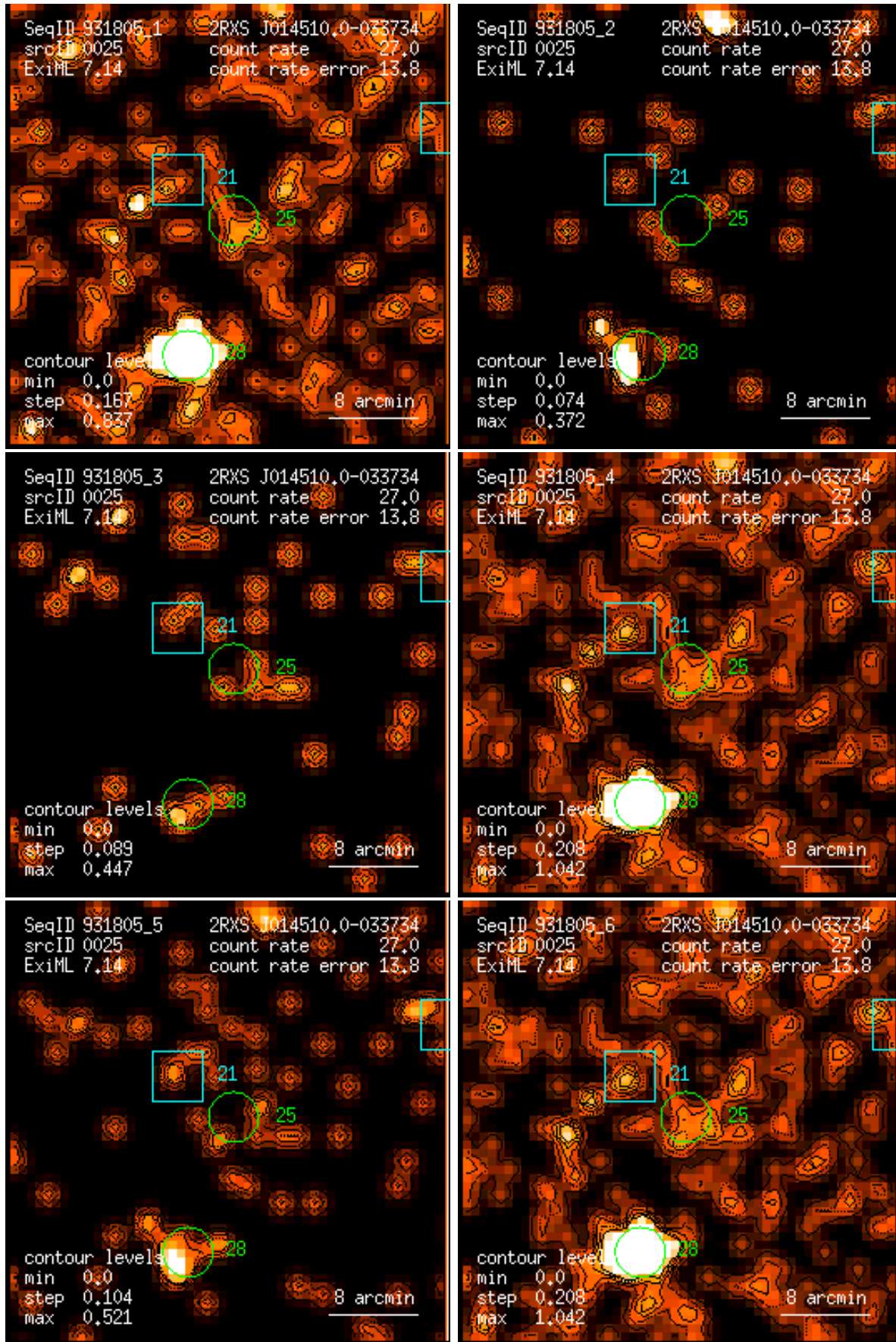
Figure 25: RASS 931805: detection 0025: band rate images, Gaussian filter: (1) PSPC channels 11 – 41, (2) 52 – 90, (3) 91 – 201, (4) 11 – 235, (5) 52 – 201, (6) 11 – 201. Broad band rates in counts/ks. Band rate contour levels in counts/ks/arcmin 2 .
