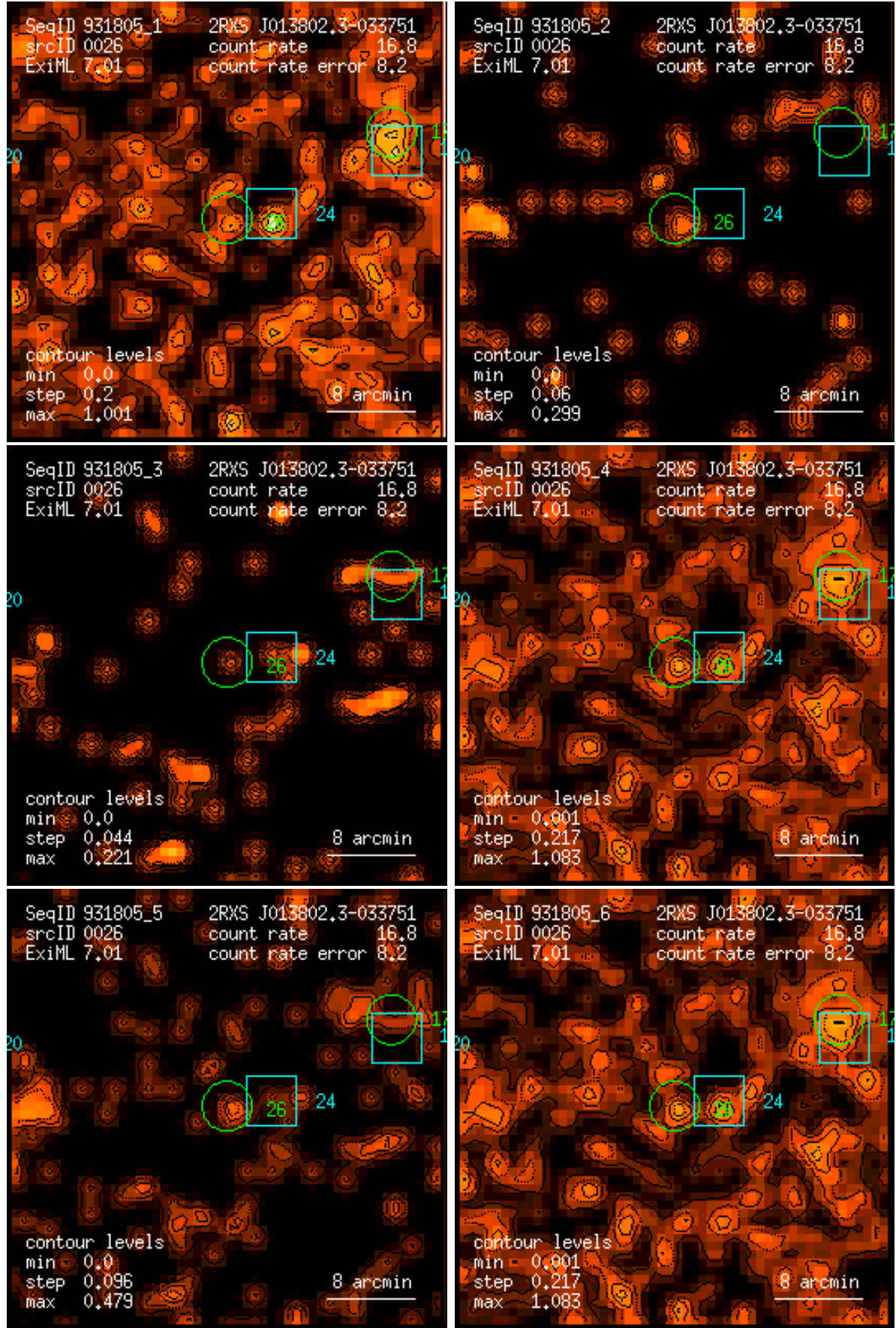
Figure 26: RASS 931805: detection 0026: band rate images, Gaussian filter: (1) PSPC channels 11 – 41, (2) 52 – 90, (3) 91 – 201, (4) 11 – 235, (5) 52 – 201, (6) 11 – 201. Broad band rates in counts/ks. Band rate contour levels in counts/ks/arcmin 2 .
