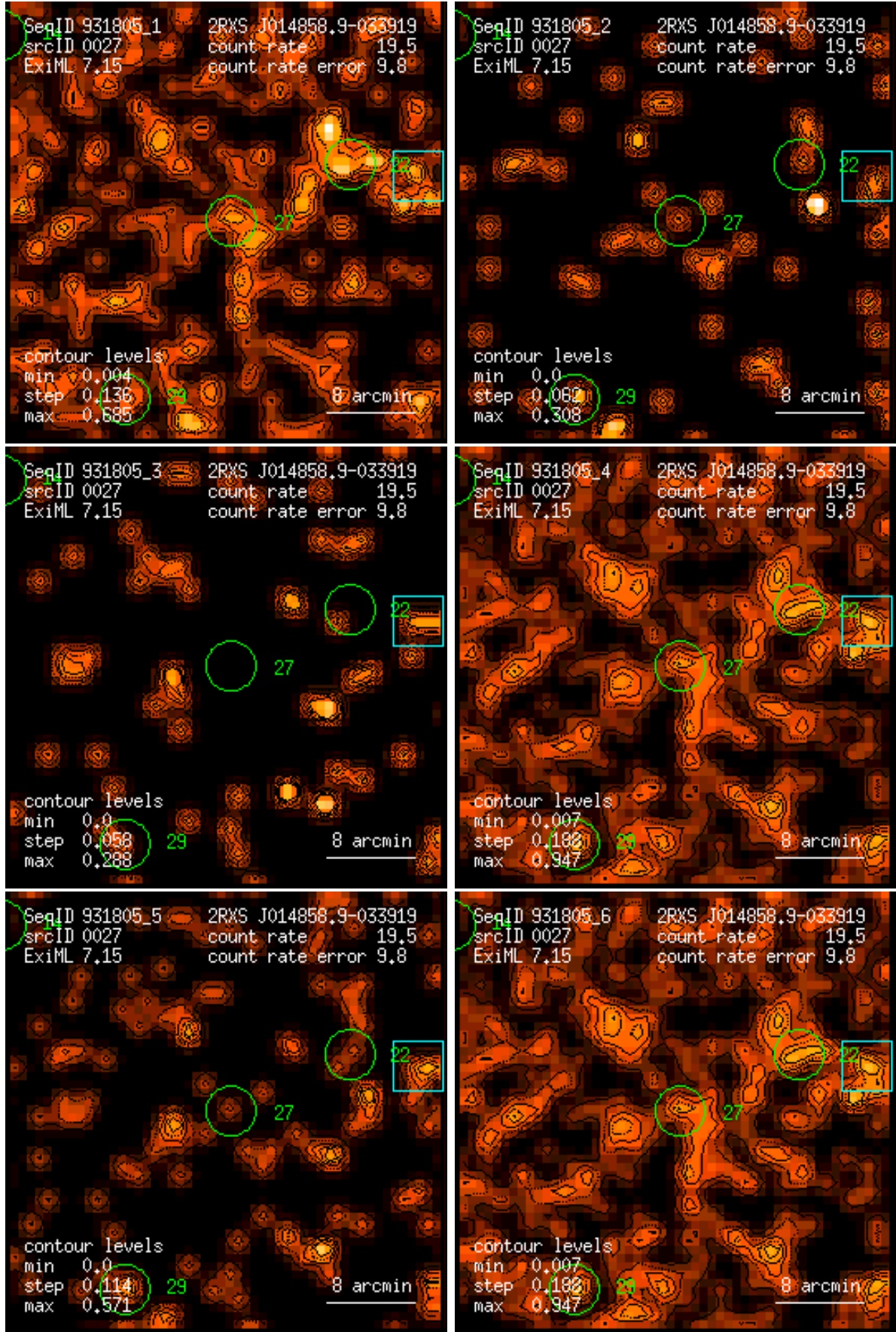
Figure 27: RASS 931805: detection 0027: band rate images, Gaussian filter: (1) PSPC channels 11 – 41, (2) 52 – 90, (3) 91 – 201, (4) 11 – 235, (5) 52 – 201, (6) 11 – 201. Broad band rates in counts/ks. Band rate contour levels in counts/ks/arcmin 2 .
