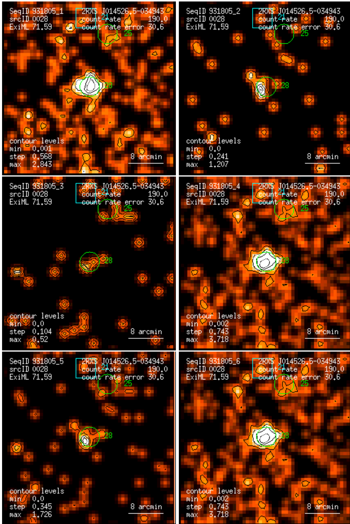
Figure 28: RASS 931805: detection 0028: band rate images, Gaussian filter: (1) PSPC channels 11 – 41, (2) 52 – 90, (3) 91 – 201, (4) 11 – 235, (5) 52 – 201, (6) 11 – 201. Broad band rates in counts/ks. Band rate contour levels in counts/ks/arcmin 2 .
