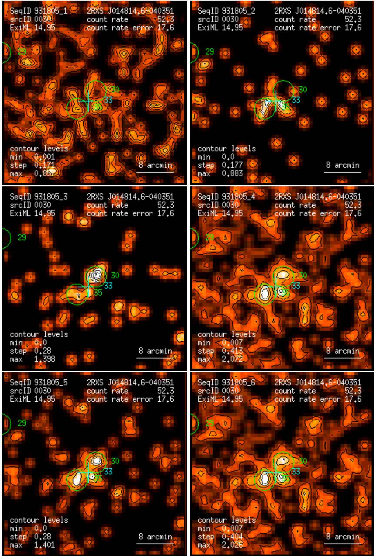
Figure 30: RASS 931805: detection 0030: band rate images, Gaussian filter: (1) PSPC channels 11 – 41, (2) 52 – 90, (3) 91 – 201, (4) 11 – 235, (5) 52 – 201, (6) 11 – 201. Broad band rates in counts/ks. Band rate contour levels in counts/ks/arcmin 2 .
