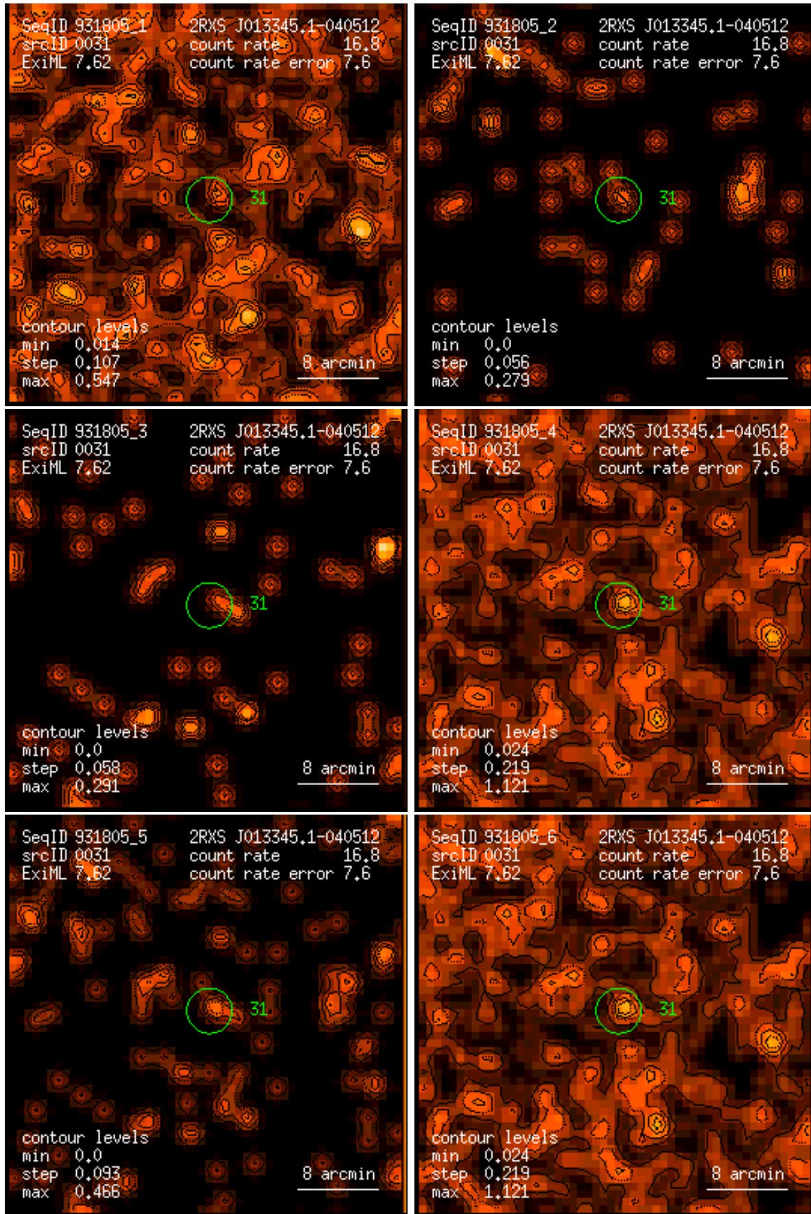
Figure 31: RASS 931805: detection 0031: band rate images, Gaussian filter: (1) PSPC channels 11 – 41, (2) 52 – 90, (3) 91 – 201, (4) 11 – 235, (5) 52 – 201, (6) 11 – 201. Broad band rates in counts/ks. Band rate contour levels in counts/ks/arcmin 2 .
