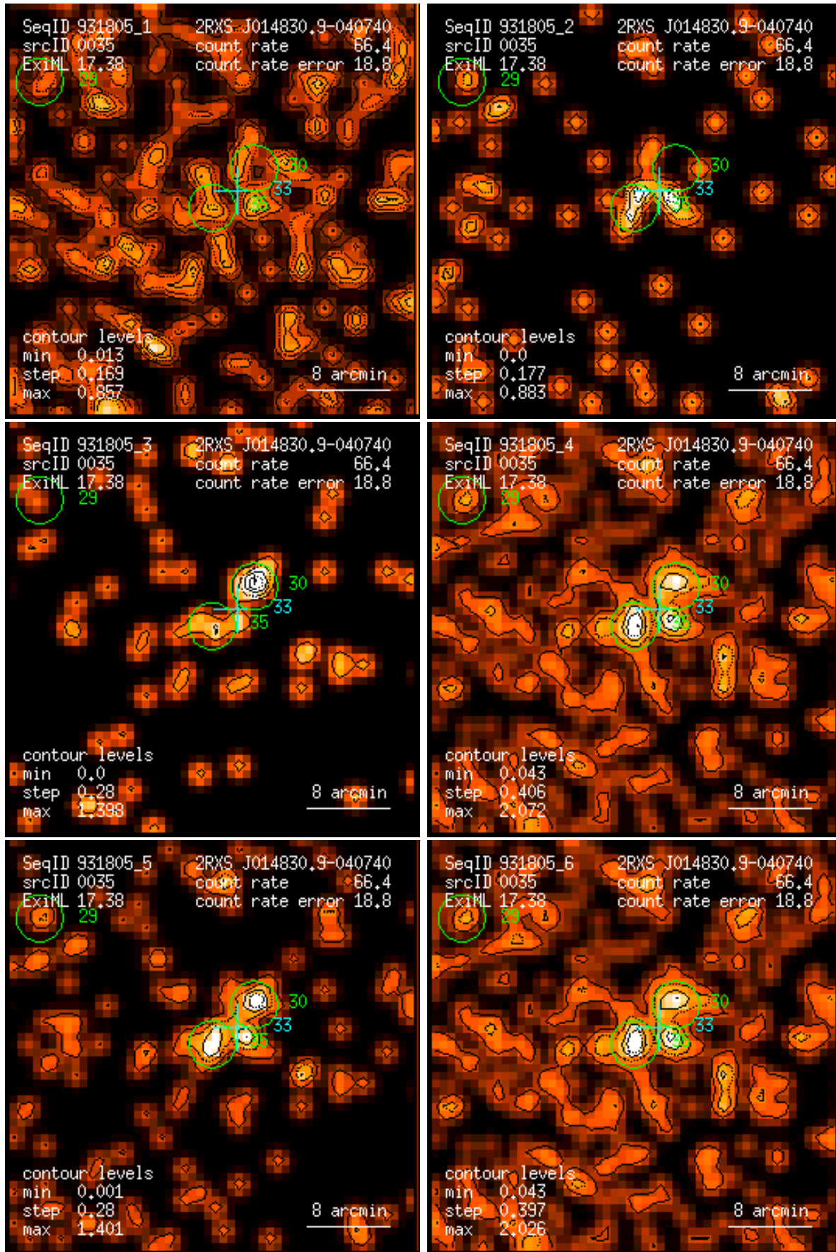
Figure 35: RASS 931805: detection 0035: band rate images, Gaussian filter: (1) PSPC channels 11 – 41, (2) 52 – 90, (3) 91 – 201, (4) 11 – 235, (5) 52 – 201, (6) 11 – 201. Broad band rates in counts/ks. Band rate contour levels in counts/ks/arcmin 2 .
