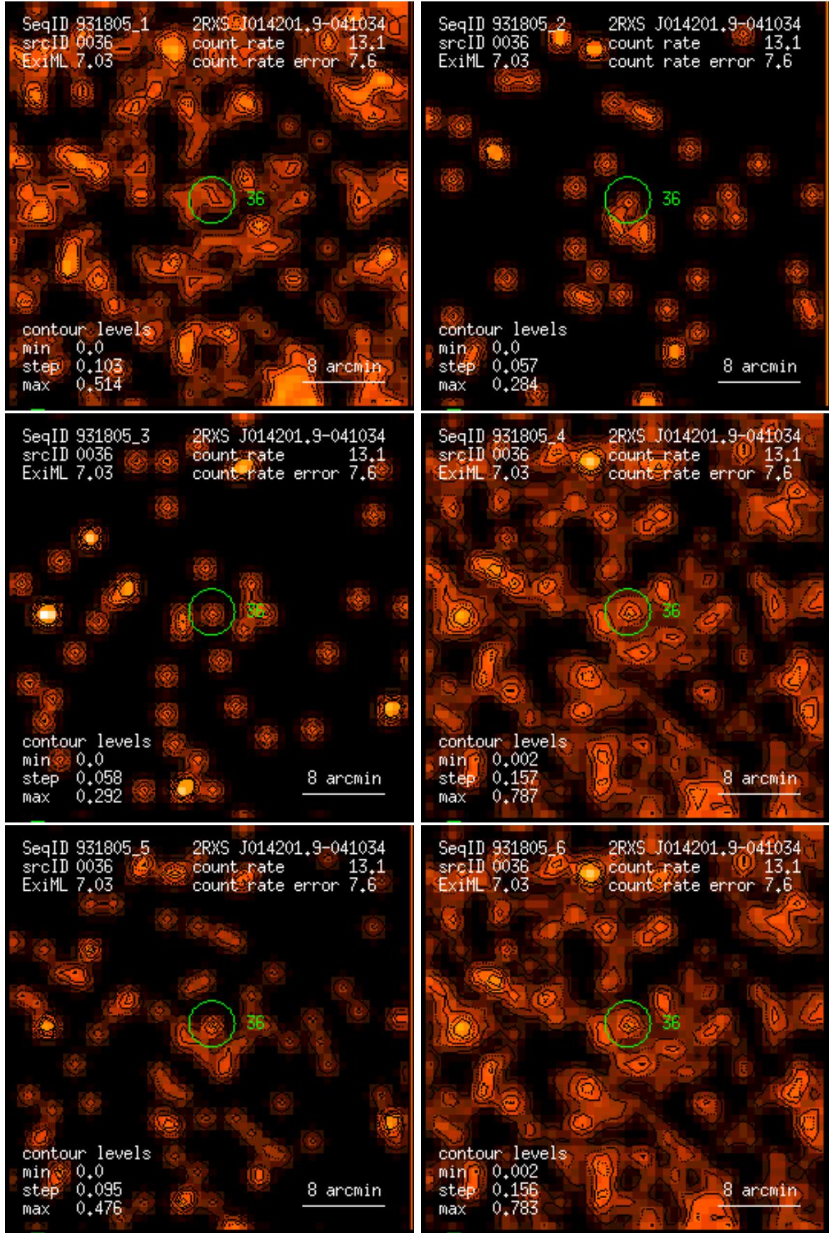
Figure 36: RASS 931805: detection 0036: band rate images, Gaussian filter: (1) PSPC channels 11 – 41, (2) 52 – 90, (3) 91 – 201, (4) 11 – 235, (5) 52 – 201, (6) 11 – 201. Broad band rates in counts/ks. Band rate contour levels in counts/ks/arcmin 2 .
