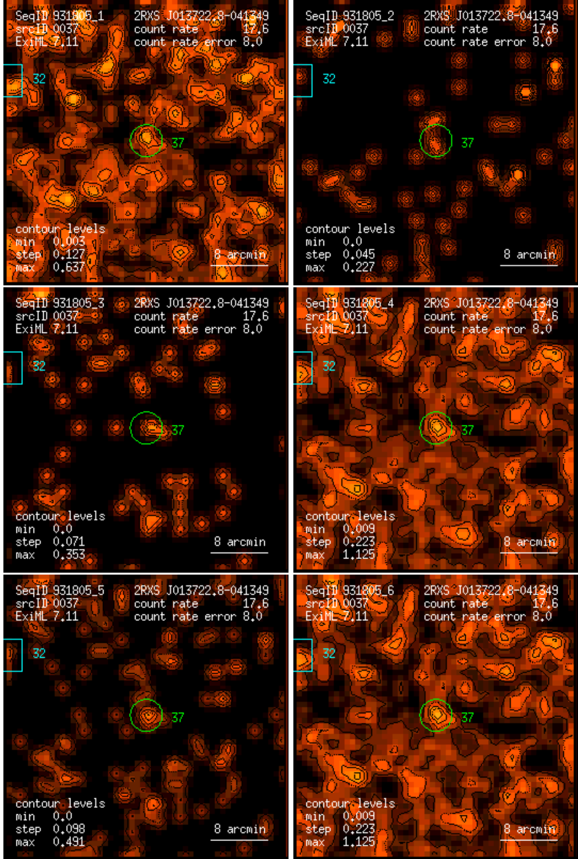
Figure 37: RASS 931805: detection 0037: band rate images, Gaussian filter: (1) PSPC channels 11 – 41, (2) 52 – 90, (3) 91 – 201, (4) 11 – 235, (5) 52 – 201, (6) 11 – 201. Broad band rates in counts/ks. Band rate contour levels in counts/ks/arcmin 2 .
