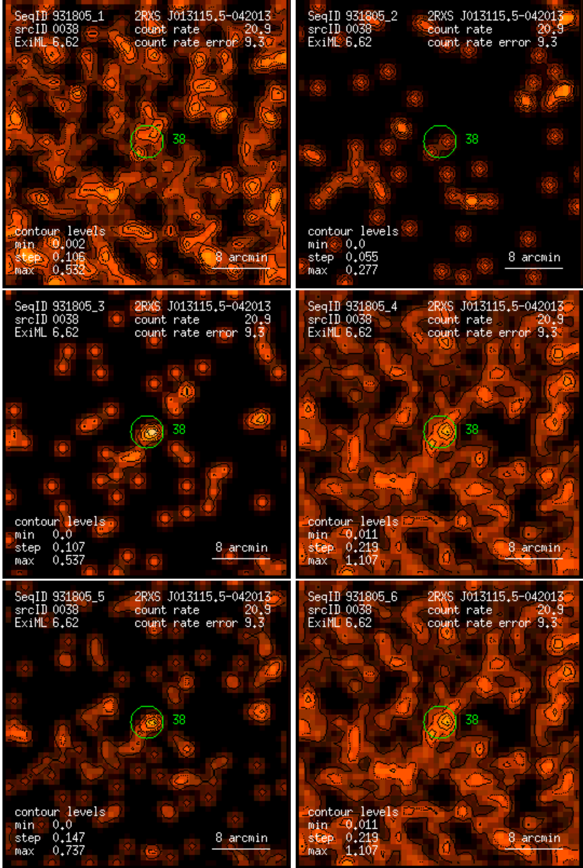
Figure 38: RASS 931805: detection 0038: band rate images, Gaussian filter: (1) PSPC channels 11 – 41, (2) 52 – 90, (3) 91 – 201, (4) 11 – 235, (5) 52 – 201, (6) 11 – 201. Broad band rates in counts/ks. Band rate contour levels in counts/ks/arcmin 2 .
