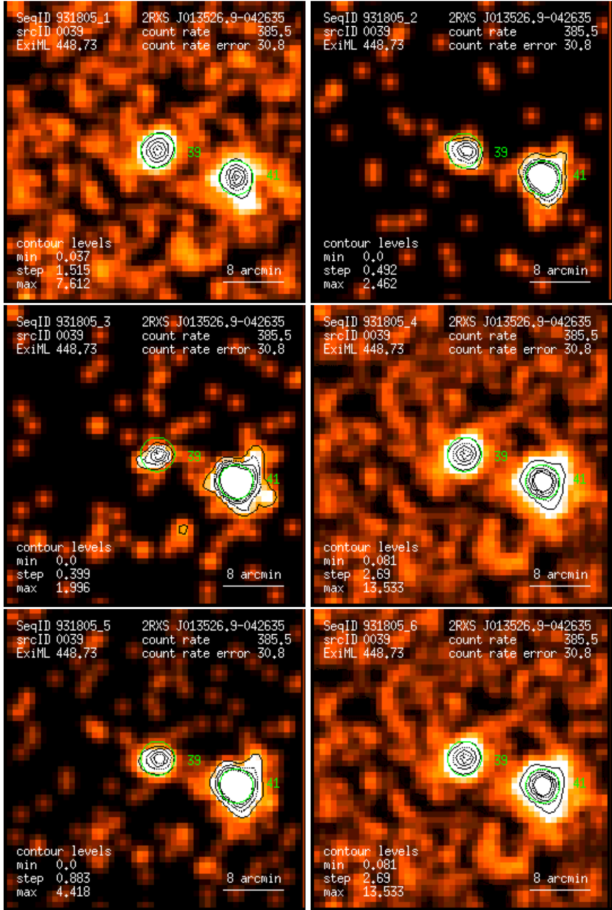
Figure 39: RASS 931805: detection 0039: band rate images, Gaussian filter: (1) PSPC channels 11 – 41, (2) 52 – 90, (3) 91 – 201, (4) 11 – 235, (5) 52 – 201, (6) 11 – 201. Broad band rates in counts/ks. Band rate contour levels in counts/ks/arcmin 2 .
