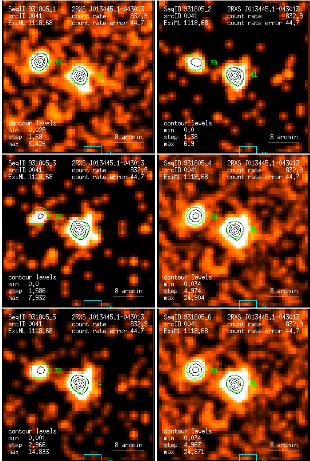
Figure 41: RASS 931805: detection 0041: band rate images, Gaussian filter: (1) PSPC channels 11 – 41, (2) 52 – 90, (3) 91 – 201, (4) 11 – 235, (5) 52 – 201, (6) 11 – 201. Broad band rates in counts/ks. Band rate contour levels in counts/ks/arcmin 2 .
