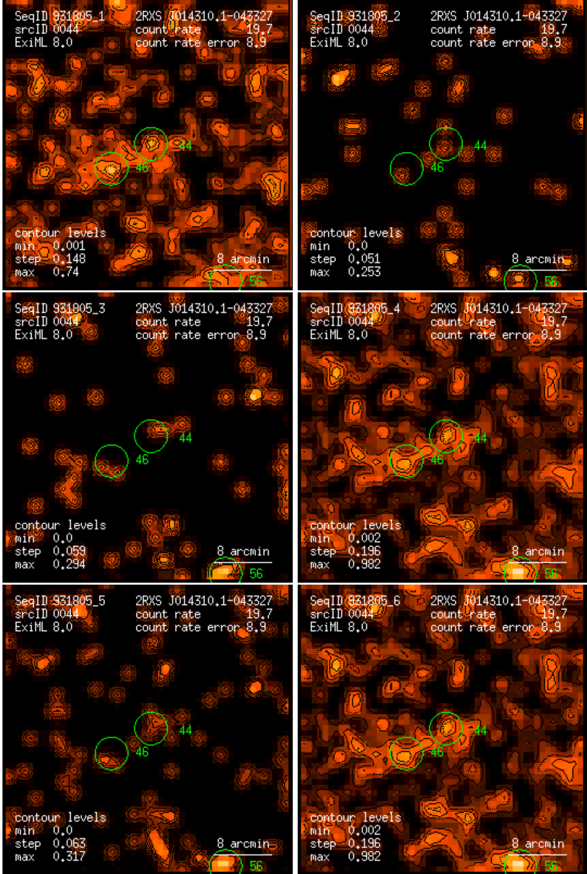
Figure 44: RASS 931805: detection 0044: band rate images, Gaussian filter: (1) PSPC channels 11 – 41, (2) 52 – 90, (3) 91 – 201, (4) 11 – 235, (5) 52 – 201, (6) 11 – 201. Broad band rates in counts/ks. Band rate contour levels in counts/ks/arcmin 2 .
