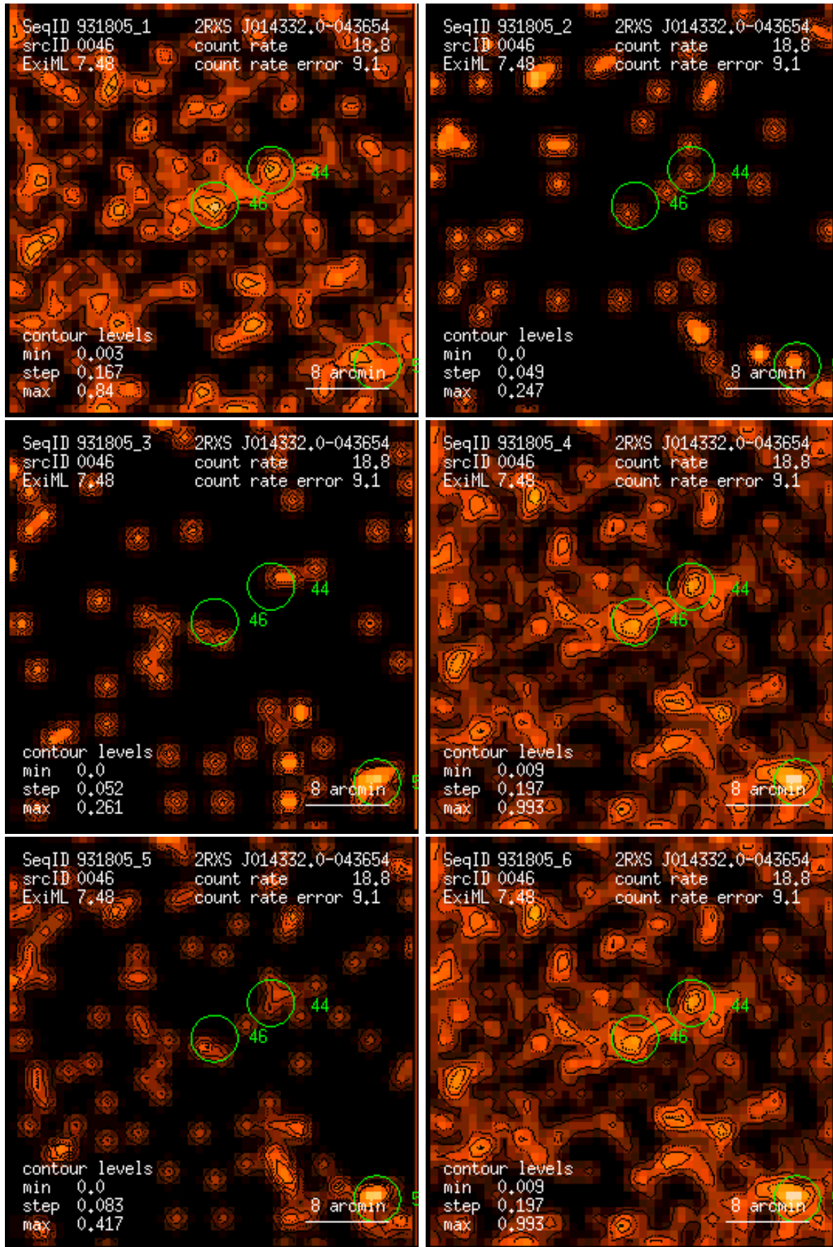
Figure 46: RASS 931805: detection 0046: band rate images, Gaussian filter: (1) PSPC channels 11 – 41, (2) 52 – 90, (3) 91 – 201, (4) 11 – 235, (5) 52 – 201, (6) 11 – 201. Broad band rates in counts/ks. Band rate contour levels in counts/ks/arcmin 2 .
