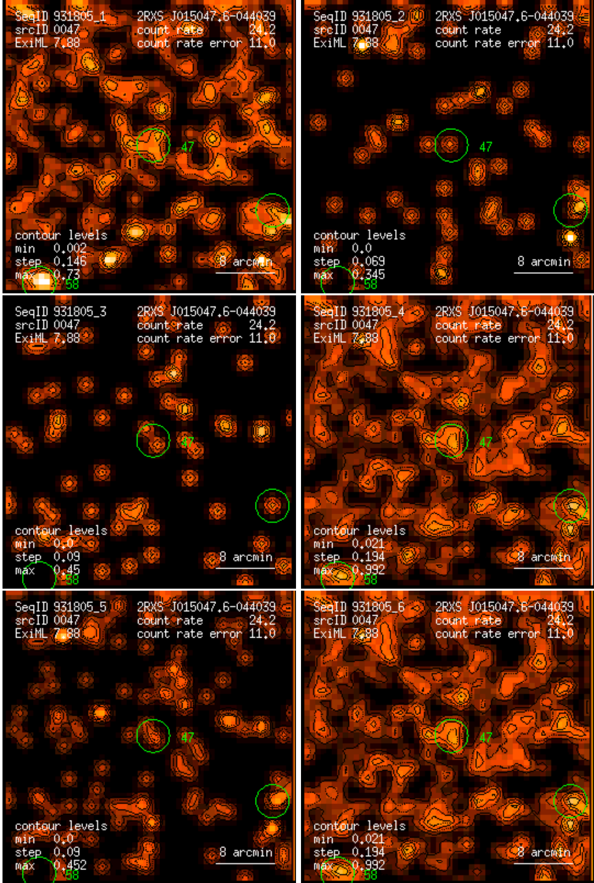
Figure 47: RASS 931805: detection 0047: band rate images, Gaussian filter: (1) PSPC channels 11 – 41, (2) 52 – 90, (3) 91 – 201, (4) 11 – 235, (5) 52 – 201, (6) 11 – 201. Broad band rates in counts/ks. Band rate contour levels in counts/ks/arcmin 2 .
