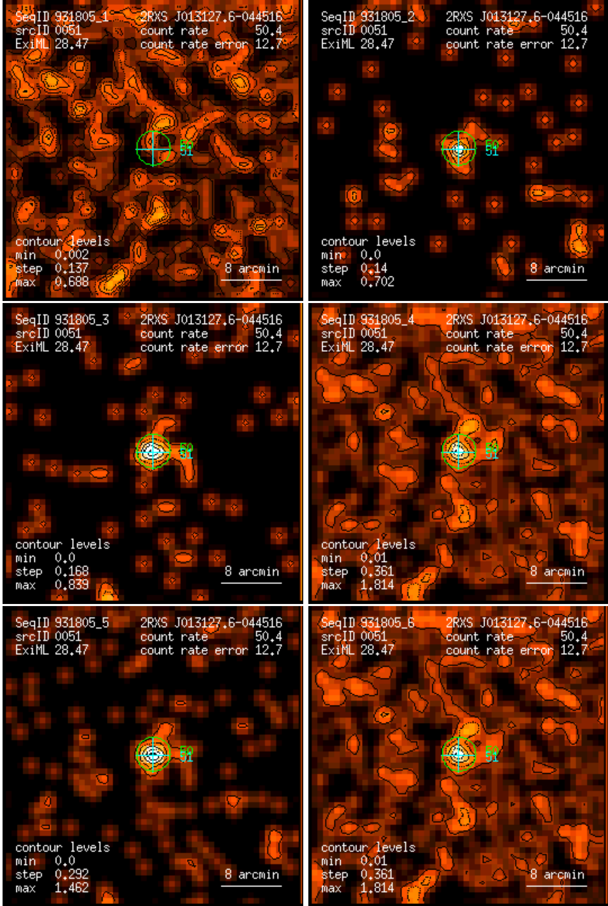
Figure 51: RASS 931805: detection 0051: band rate images, Gaussian filter: (1) PSPC channels 11 – 41, (2) 52 – 90, (3) 91 – 201, (4) 11 – 235, (5) 52 – 201, (6) 11 – 201. Broad band rates in counts/ks. Band rate contour levels in counts/ks/arcmin 2 .
