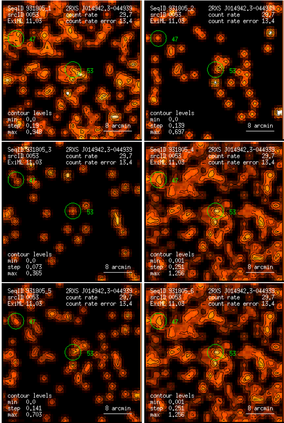
Figure 53: RASS 931805: detection 0053: band rate images, Gaussian filter: (1) PSPC channels 11 – 41, (2) 52 – 90, (3) 91 – 201, (4) 11 – 235, (5) 52 – 201, (6) 11 – 201. Broad band rates in counts/ks. Band rate contour levels in counts/ks/arcmin 2 .
