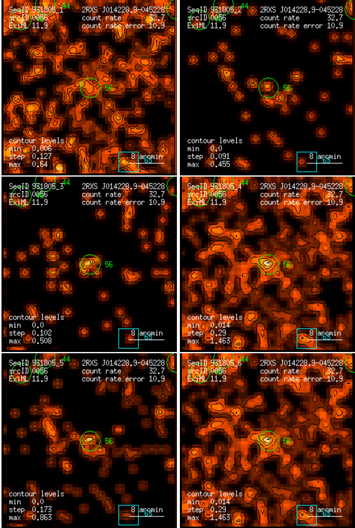
Figure 56: RASS 931805: detection 0056: band rate images, Gaussian filter: (1) PSPC channels 11 – 41, (2) 52 – 90, (3) 91 – 201, (4) 11 – 235, (5) 52 – 201, (6) 11 – 201. Broad band rates in counts/ks. Band rate contour levels in counts/ks/arcmin 2 .
