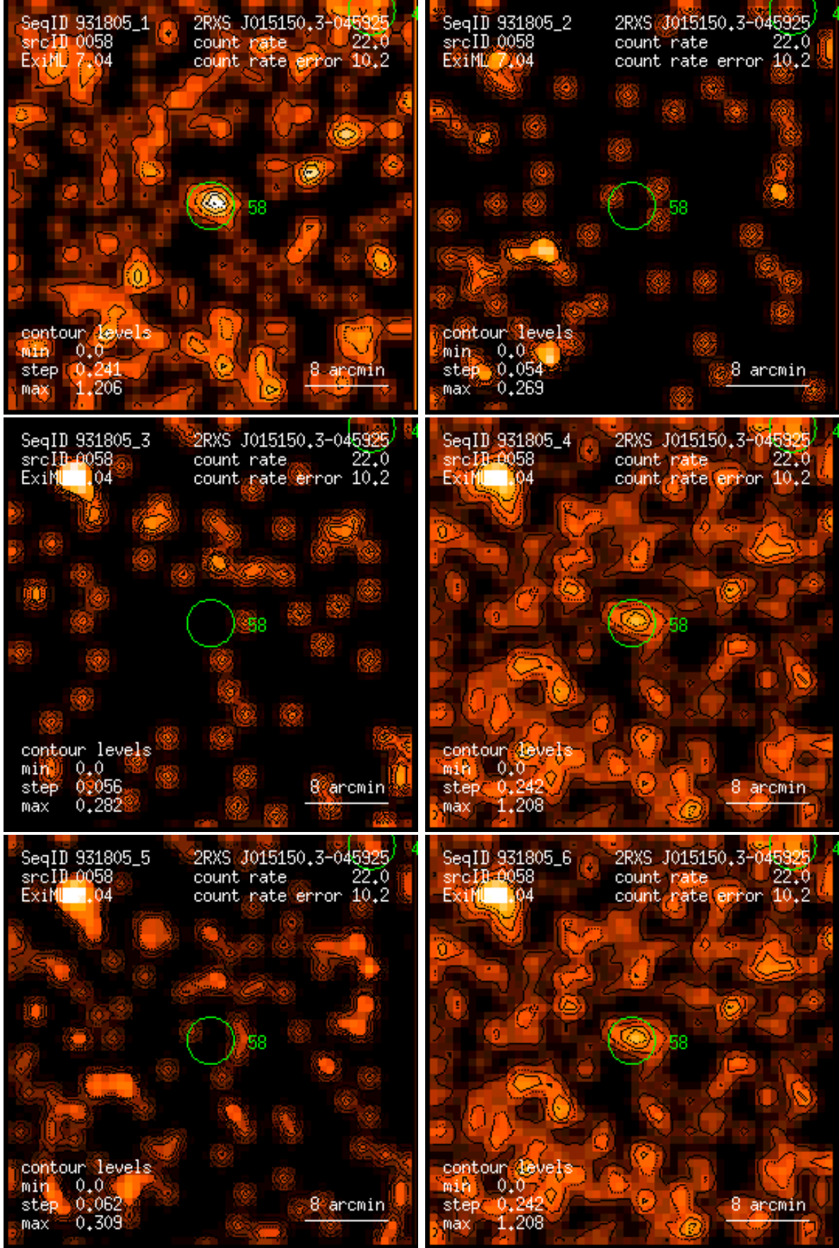
Figure 58: RASS 931805: detection 0058: band rate images, Gaussian filter: (1) PSPC channels 11 – 41, (2) 52 – 90, (3) 91 – 201, (4) 11 – 235, (5) 52 – 201, (6) 11 – 201. Broad band rates in counts/ks. Band rate contour levels in counts/ks/arcmin 2 .
