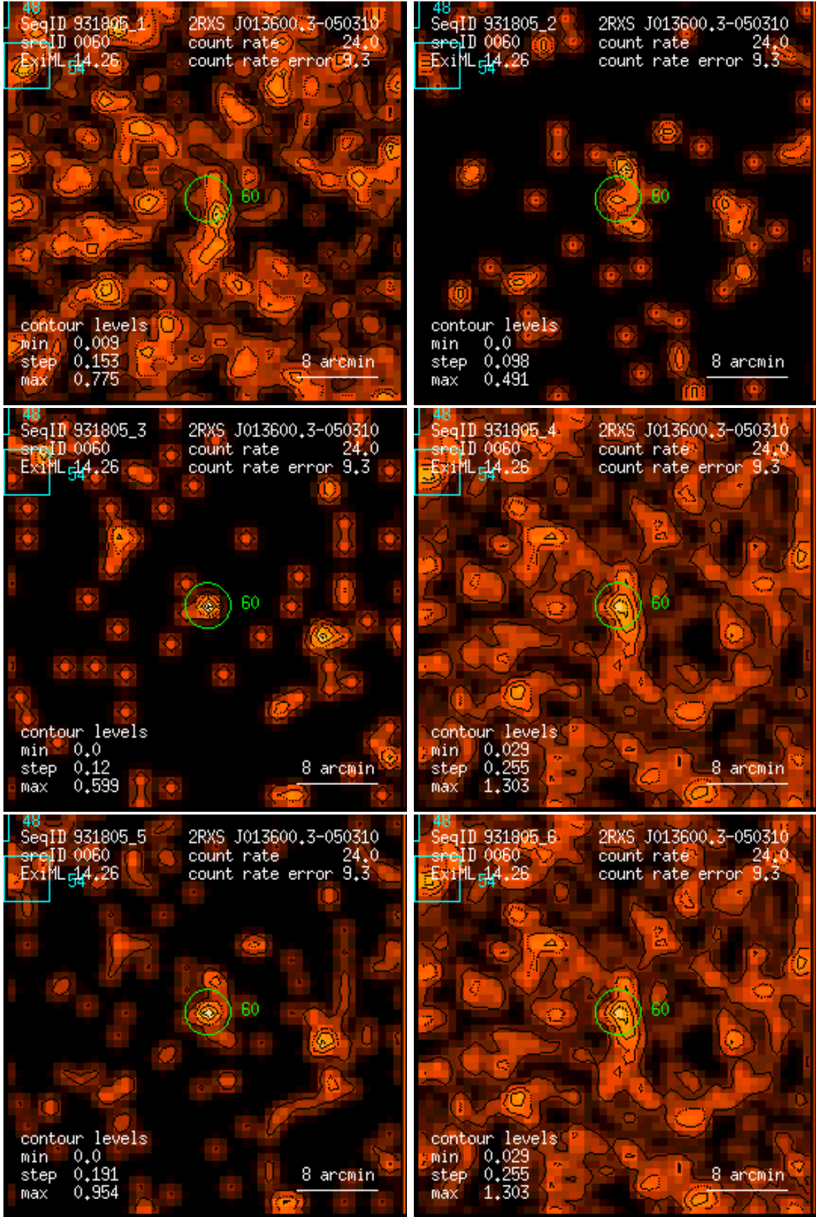
Figure 60: RASS 931805: detection 0060: band rate images, Gaussian filter: (1) PSPC channels 11 – 41, (2) 52 – 90, (3) 91 – 201, (4) 11 – 235, (5) 52 – 201, (6) 11 – 201. Broad band rates in counts/ks. Band rate contour levels in counts/ks/arcmin 2 .
