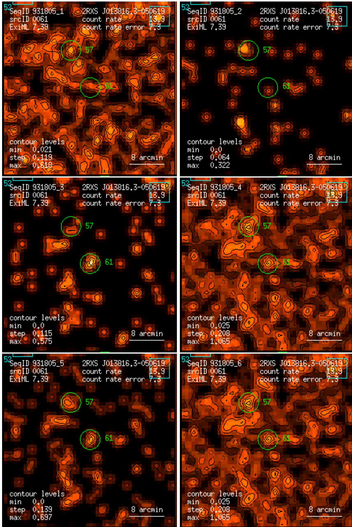
Figure 61: RASS 931805: detection 0061: band rate images, Gaussian filter: (1) PSPC channels 11 – 41, (2) 52 – 90, (3) 91 – 201, (4) 11 – 235, (5) 52 – 201, (6) 11 – 201. Broad band rates in counts/ks. Band rate contour levels in counts/ks/arcmin 2 .
