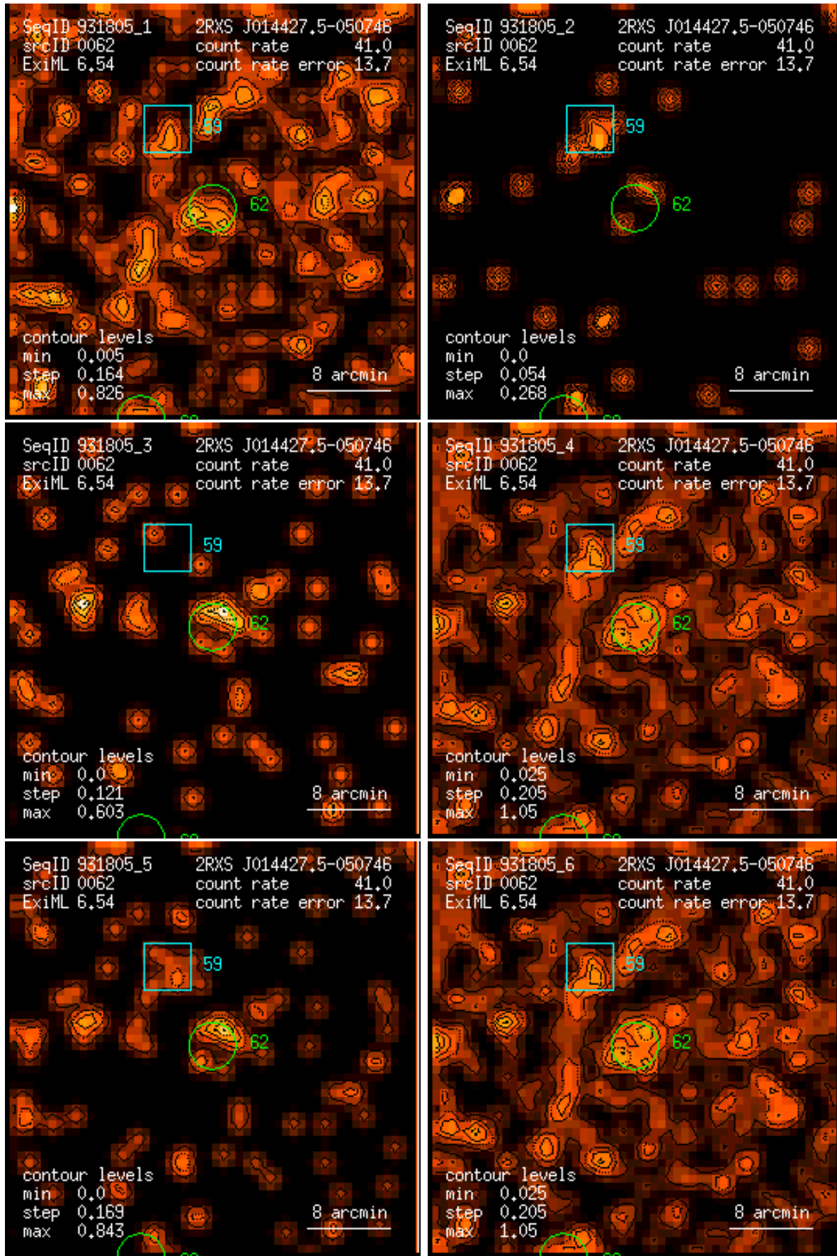
Figure 62: RASS 931805: detection 0062: band rate images, Gaussian filter: (1) PSPC channels 11 – 41, (2) 52 – 90, (3) 91 – 201, (4) 11 – 235, (5) 52 – 201, (6) 11 – 201. Broad band rates in counts/ks. Band rate contour levels in counts/ks/arcmin 2 .
