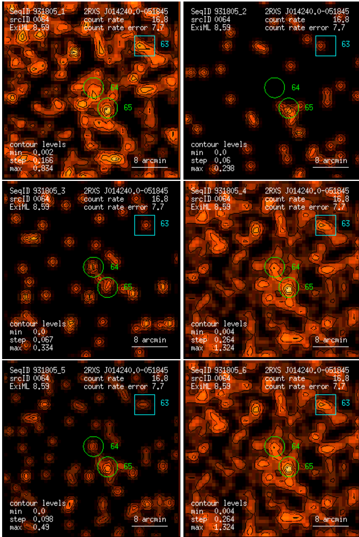
Figure 64: RASS 931805: detection 0064: band rate images, Gaussian filter: (1) PSPC channels 11 – 41, (2) 52 – 90, (3) 91 – 201, (4) 11 – 235, (5) 52 – 201, (6) 11 – 201. Broad band rates in counts/ks. Band rate contour levels in counts/ks/arcmin 2 .
