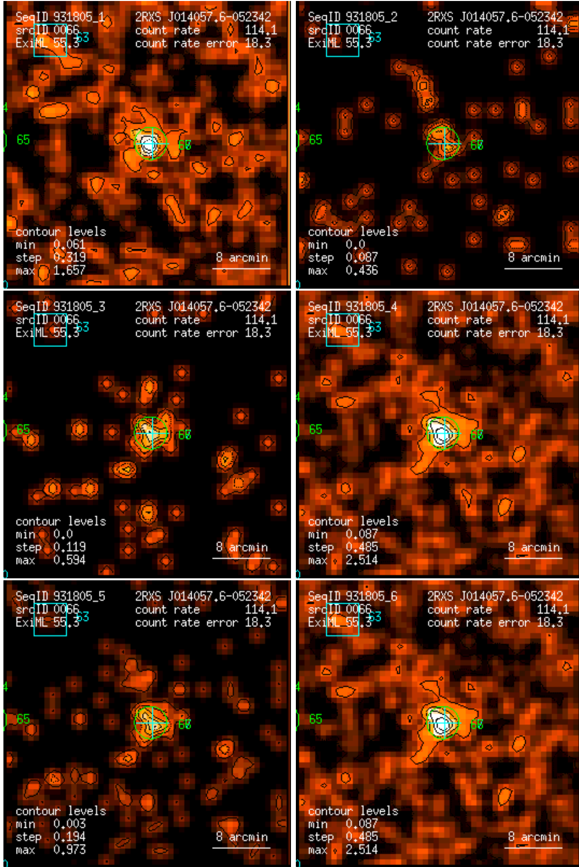
Figure 66: RASS 931805: detection 0066: band rate images, Gaussian filter: (1) PSPC channels 11 – 41, (2) 52 – 90, (3) 91 – 201, (4) 11 – 235, (5) 52 – 201, (6) 11 – 201. Broad band rates in counts/ks. Band rate contour levels in counts/ks/arcmin 2 .
