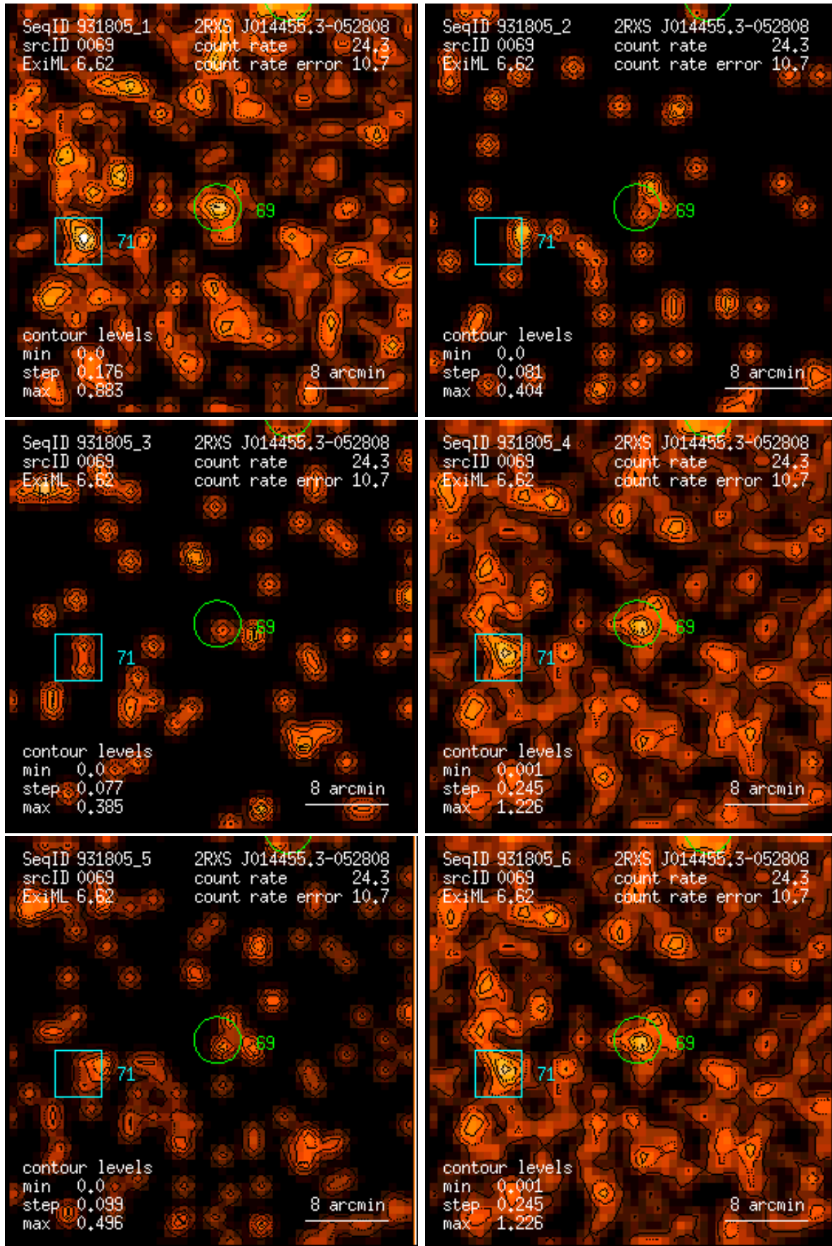
Figure 69: RASS 931805: detection 0069: band rate images, Gaussian filter: (1) PSPC channels 11 – 41, (2) 52 – 90, (3) 91 – 201, (4) 11 – 235, (5) 52 – 201, (6) 11 – 201. Broad band rates in counts/ks. Band rate contour levels in counts/ks/arcmin 2 .
