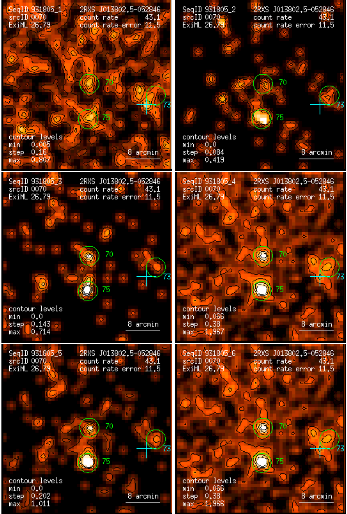
Figure 70: RASS 931805: detection 0070: band rate images, Gaussian filter: (1) PSPC channels 11 – 41, (2) 52 – 90, (3) 91 – 201, (4) 11 – 235, (5) 52 – 201, (6) 11 – 201. Broad band rates in counts/ks. Band rate contour levels in counts/ks/arcmin 2 .
