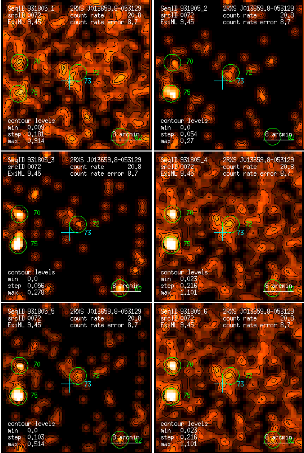
Figure 72: RASS 931805: detection 0072: band rate images, Gaussian filter: (1) PSPC channels 11 – 41, (2) 52 – 90, (3) 91 – 201, (4) 11 – 235, (5) 52 – 201, (6) 11 – 201. Broad band rates in counts/ks. Band rate contour levels in counts/ks/arcmin 2 .
