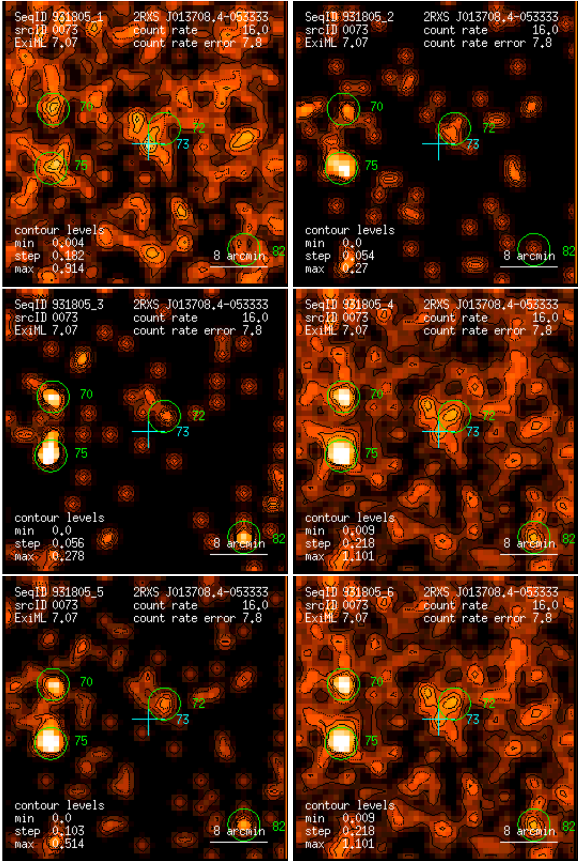
Figure 73: RASS 931805: detection 0073: band rate images, Gaussian filter: (1) PSPC channels 11 – 41, (2) 52 – 90, (3) 91 – 201, (4) 11 – 235, (5) 52 – 201, (6) 11 – 201. Broad band rates in counts/ks. Band rate contour levels in counts/ks/arcmin 2 .
