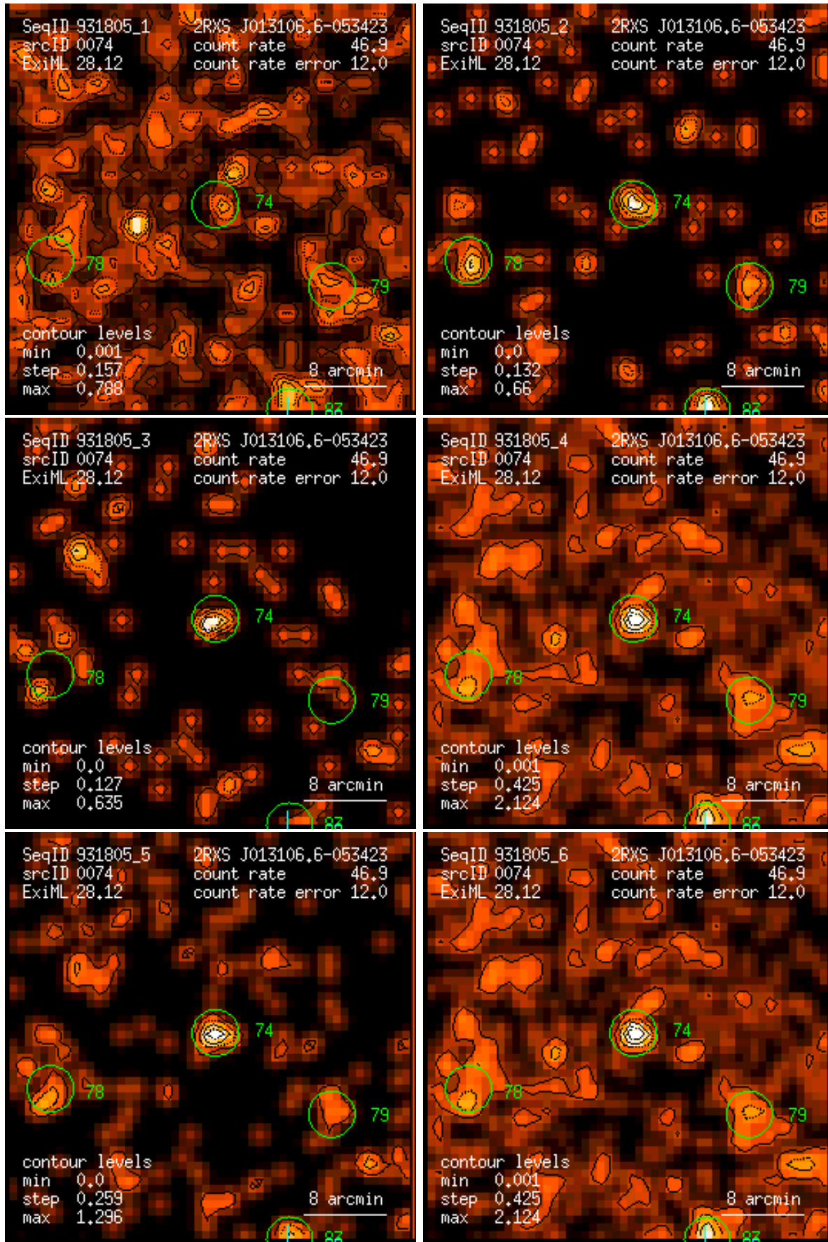
Figure 74: RASS 931805: detection 0074: band rate images, Gaussian filter: (1) PSPC channels 11 – 41, (2) 52 – 90, (3) 91 – 201, (4) 11 – 235, (5) 52 – 201, (6) 11 – 201. Broad band rates in counts/ks. Band rate contour levels in counts/ks/arcmin 2 .
