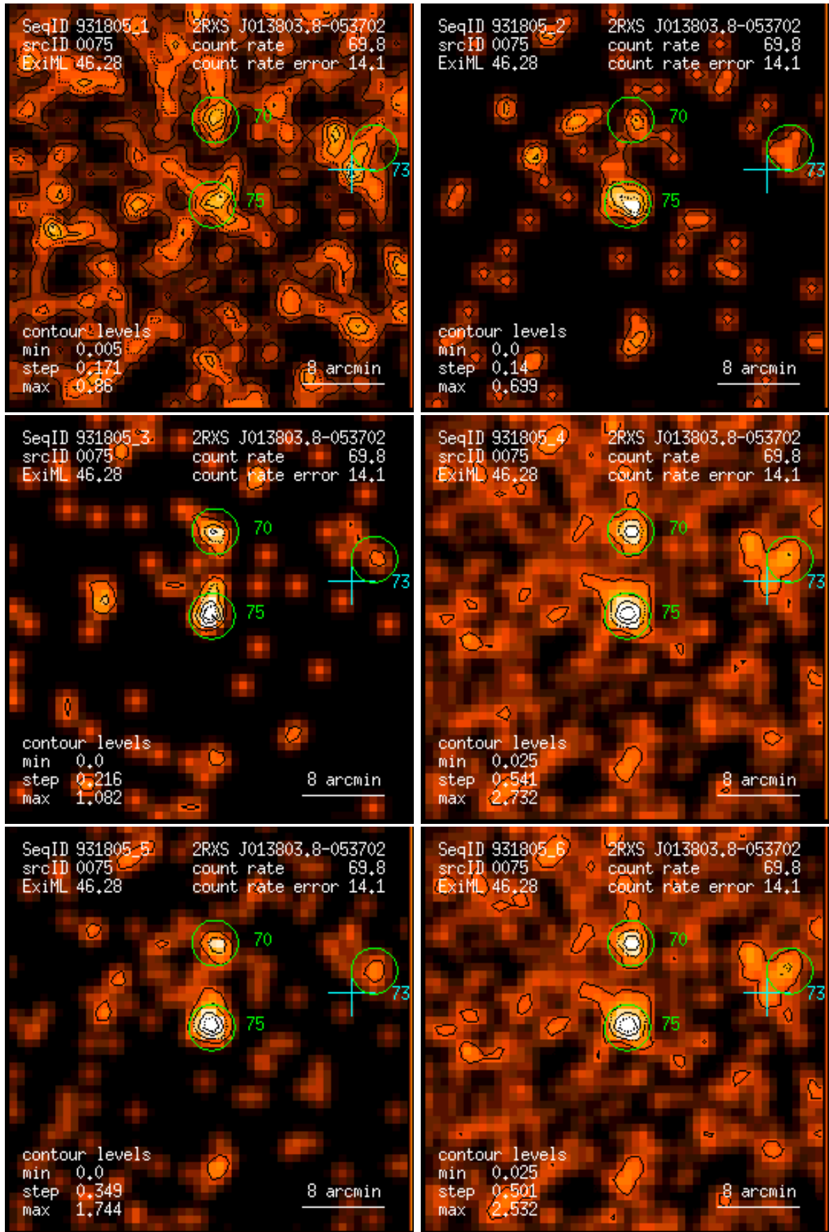
Figure 75: RASS 931805: detection 0075: band rate images, Gaussian filter: (1) PSPC channels 11 – 41, (2) 52 – 90, (3) 91 – 201, (4) 11 – 235, (5) 52 – 201, (6) 11 – 201. Broad band rates in counts/ks. Band rate contour levels in counts/ks/arcmin 2 .
