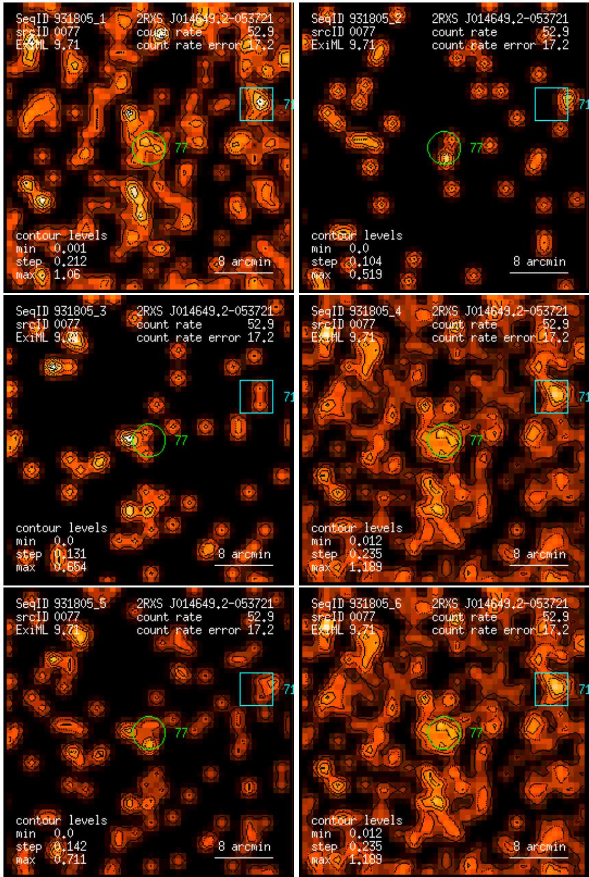
Figure 77: RASS 931805: detection 0077: band rate images, Gaussian filter: (1) PSPC channels 11 – 41, (2) 52 – 90, (3) 91 – 201, (4) 11 – 235, (5) 52 – 201, (6) 11 – 201. Broad band rates in counts/ks. Band rate contour levels in counts/ks/arcmin 2 .
