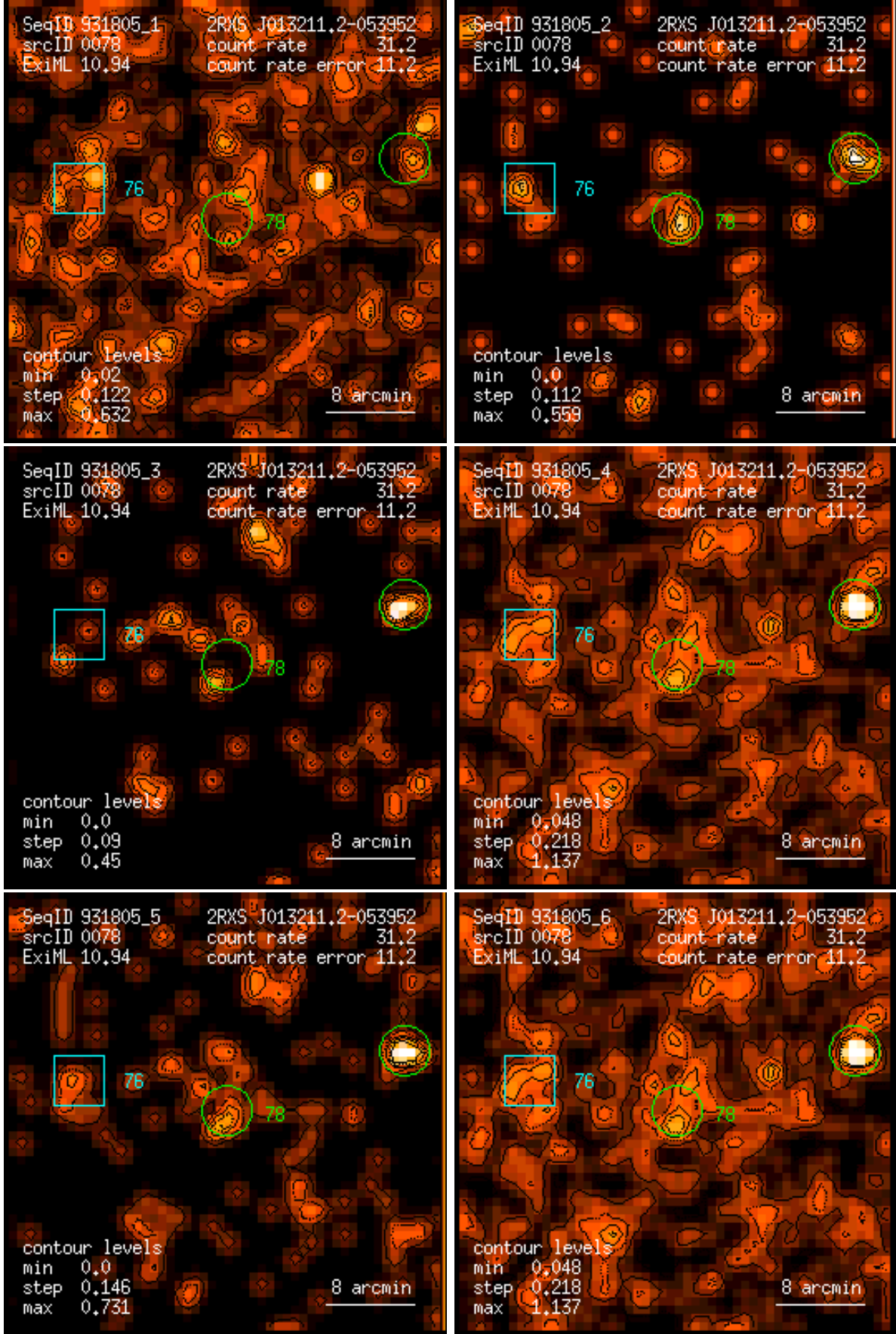
Figure 78: RASS 931805: detection 0078: band rate images, Gaussian filter: (1) PSPC channels 11 – 41, (2) 52 – 90, (3) 91 – 201, (4) 11 – 235, (5) 52 – 201, (6) 11 – 201. Broad band rates in counts/ks. Band rate contour levels in counts/ks/arcmin 2 .
