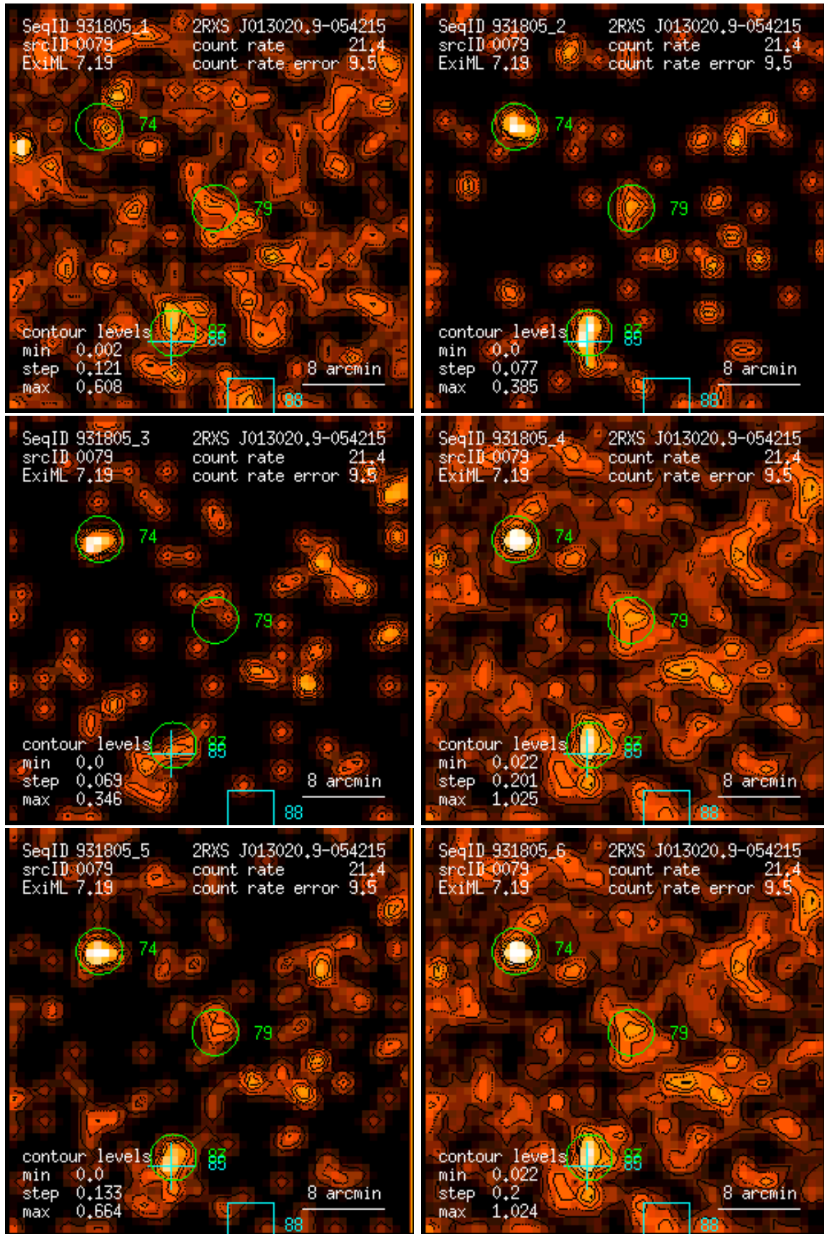
Figure 79: RASS 931805: detection 0079: band rate images, Gaussian filter: (1) PSPC channels 11 – 41, (2) 52 – 90, (3) 91 – 201, (4) 11 – 235, (5) 52 – 201, (6) 11 – 201. Broad band rates in counts/ks. Band rate contour levels in counts/ks/arcmin 2 .
