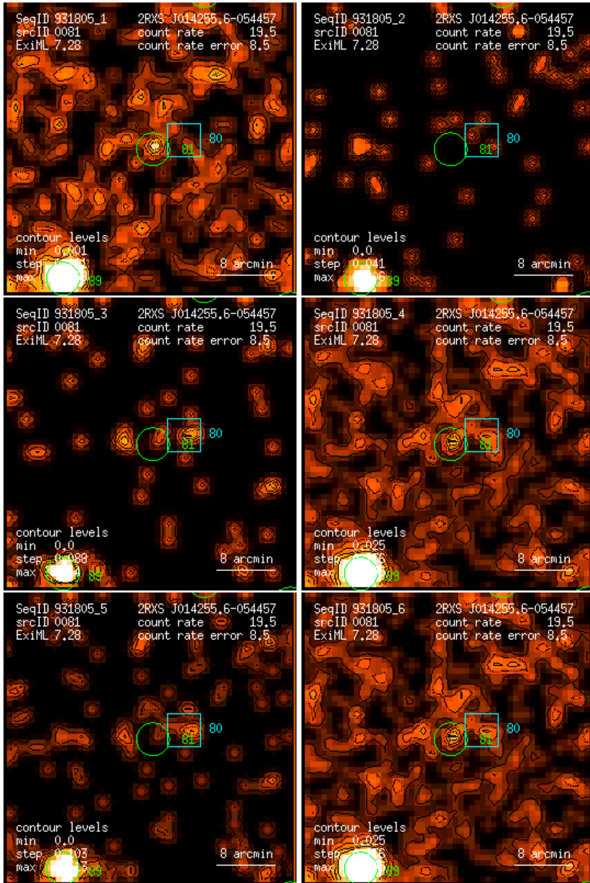
Figure 81: RASS 931805: detection 0081: band rate images, Gaussian filter: (1) PSPC channels 11 – 41, (2) 52 – 90, (3) 91 – 201, (4) 11 – 235, (5) 52 – 201, (6) 11 – 201. Broad band rates in counts/ks. Band rate contour levels in counts/ks/arcmin 2 .
