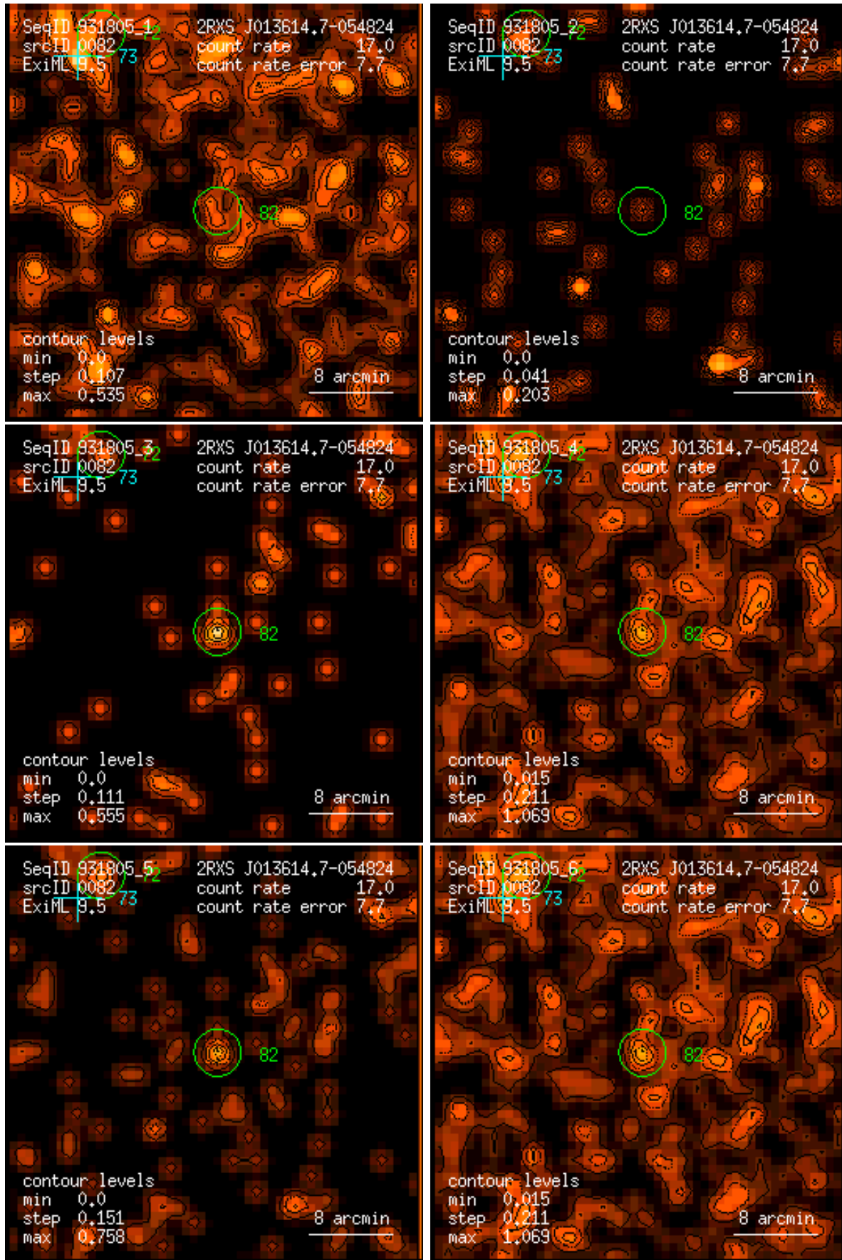
Figure 82: RASS 931805: detection 0082: band rate images, Gaussian filter: (1) PSPC channels 11 – 41, (2) 52 – 90, (3) 91 – 201, (4) 11 – 235, (5) 52 – 201, (6) 11 – 201. Broad band rates in counts/ks. Band rate contour levels in counts/ks/arcmin 2 .
