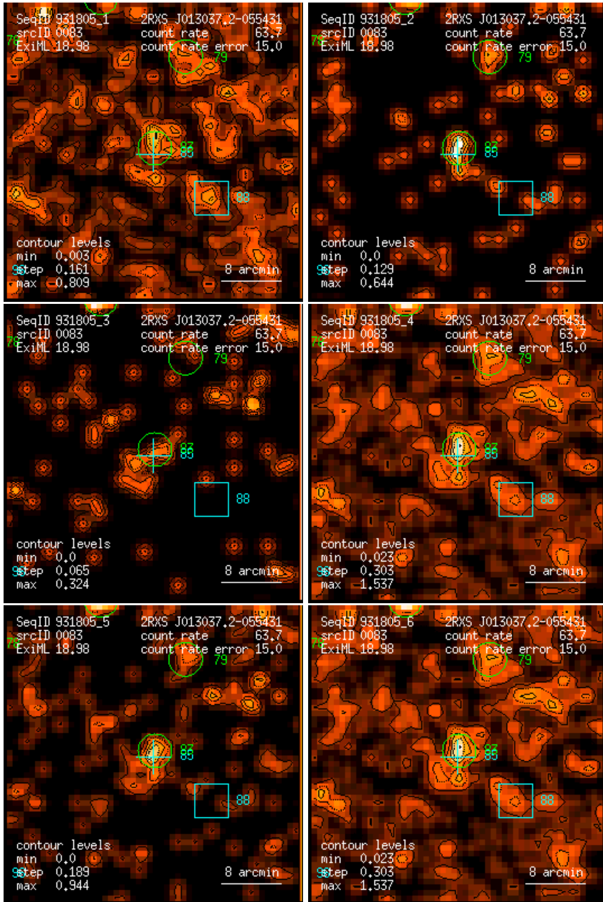
Figure 83: RASS 931805: detection 0083: band rate images, Gaussian filter: (1) PSPC channels 11 – 41, (2) 52 – 90, (3) 91 – 201, (4) 11 – 235, (5) 52 – 201, (6) 11 – 201. Broad band rates in counts/ks. Band rate contour levels in counts/ks/arcmin 2 .
