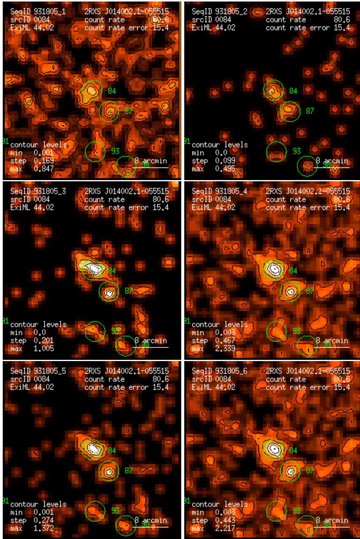
Figure 84: RASS 931805: detection 0084: band rate images, Gaussian filter: (1) PSPC channels 11 – 41, (2) 52 – 90, (3) 91 – 201, (4) 11 – 235, (5) 52 – 201, (6) 11 – 201. Broad band rates in counts/ks. Band rate contour levels in counts/ks/arcmin 2 .
