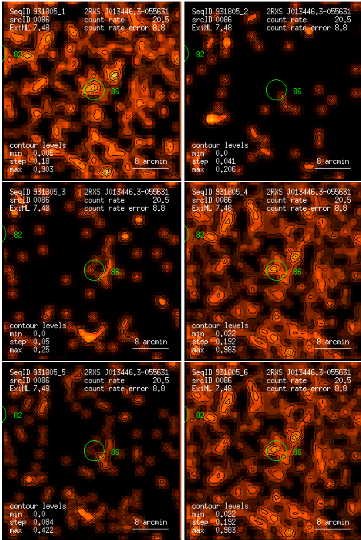
Figure 86: RASS 931805: detection 0086: band rate images, Gaussian filter: (1) PSPC channels 11 – 41, (2) 52 – 90, (3) 91 – 201, (4) 11 – 235, (5) 52 – 201, (6) 11 – 201. Broad band rates in counts/ks. Band rate contour levels in counts/ks/arcmin 2 .
