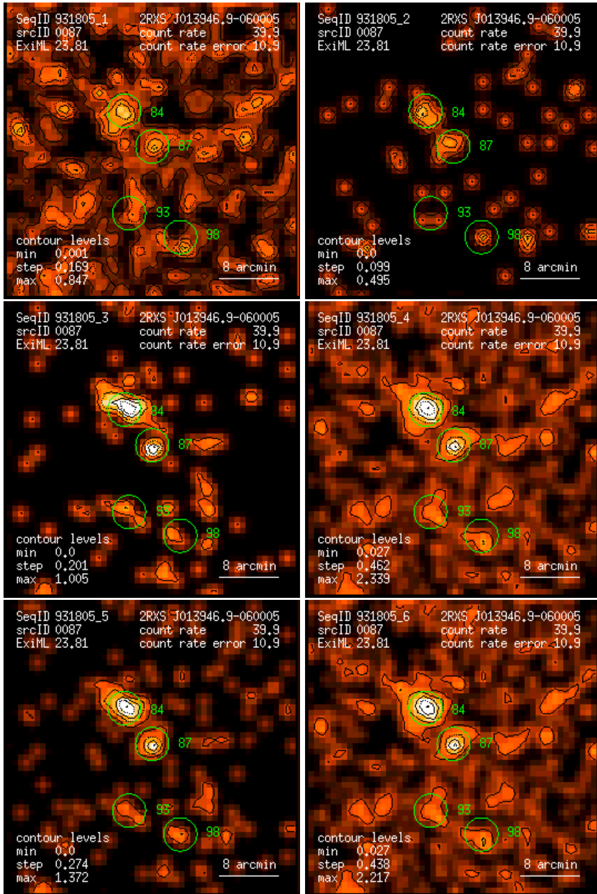
Figure 87: RASS 931805: detection 0087: band rate images, Gaussian filter: (1) PSPC channels 11 – 41, (2) 52 – 90, (3) 91 – 201, (4) 11 – 235, (5) 52 – 201, (6) 11 – 201. Broad band rates in counts/ks. Band rate contour levels in counts/ks/arcmin 2 .
