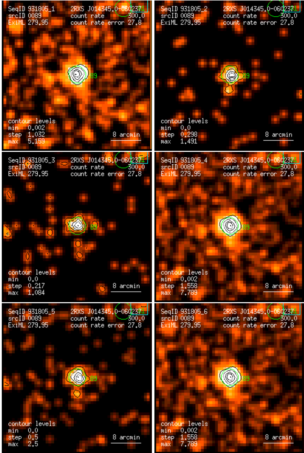
Figure 89: RASS 931805: detection 0089: band rate images, Gaussian filter: (1) PSPC channels 11 – 41, (2) 52 – 90, (3) 91 – 201, (4) 11 – 235, (5) 52 – 201, (6) 11 – 201. Broad band rates in counts/ks. Band rate contour levels in counts/ks/arcmin 2 .
