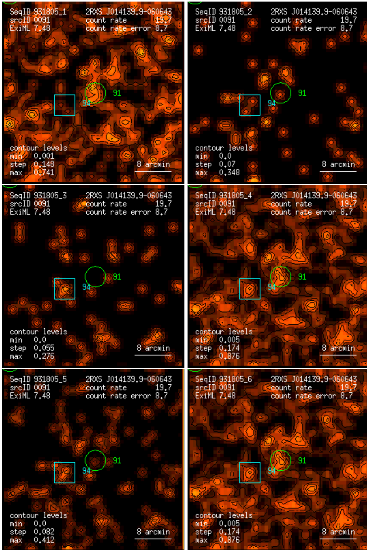
Figure 91: RASS 931805: detection 0091: band rate images, Gaussian filter: (1) PSPC channels 11 – 41, (2) 52 – 90, (3) 91 – 201, (4) 11 – 235, (5) 52 – 201, (6) 11 – 201. Broad band rates in counts/ks. Band rate contour levels in counts/ks/arcmin 2 .
