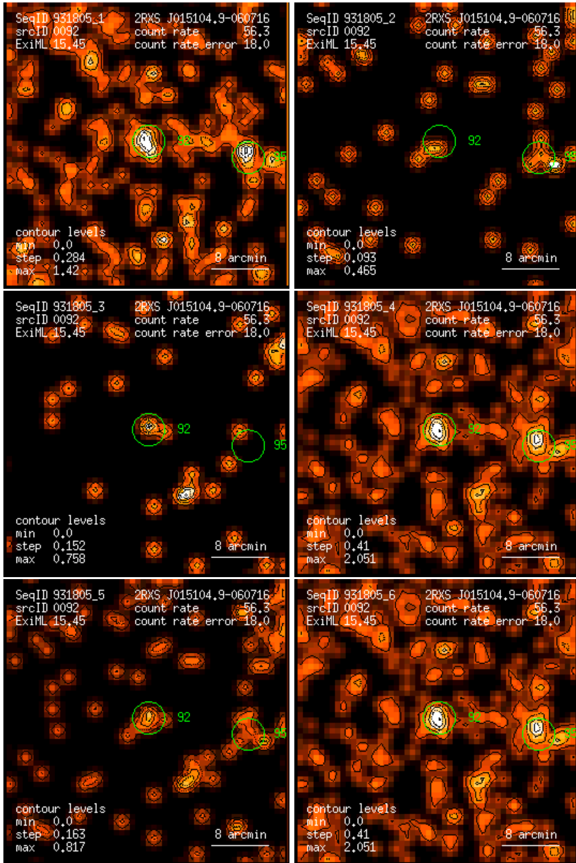
Figure 92: RASS 931805: detection 0092: band rate images, Gaussian filter: (1) PSPC channels 11 – 41, (2) 52 – 90, (3) 91 – 201, (4) 11 – 235, (5) 52 – 201, (6) 11 – 201. Broad band rates in counts/ks. Band rate contour levels in counts/ks/arcmin 2 .
