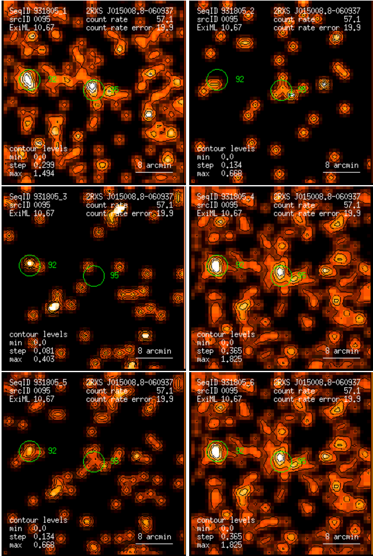
Figure 95: RASS 931805: detection 0095: band rate images, Gaussian filter: (1) PSPC channels 11 – 41, (2) 52 – 90, (3) 91 – 201, (4) 11 – 235, (5) 52 – 201, (6) 11 – 201. Broad band rates in counts/ks. Band rate contour levels in counts/ks/arcmin 2 .
