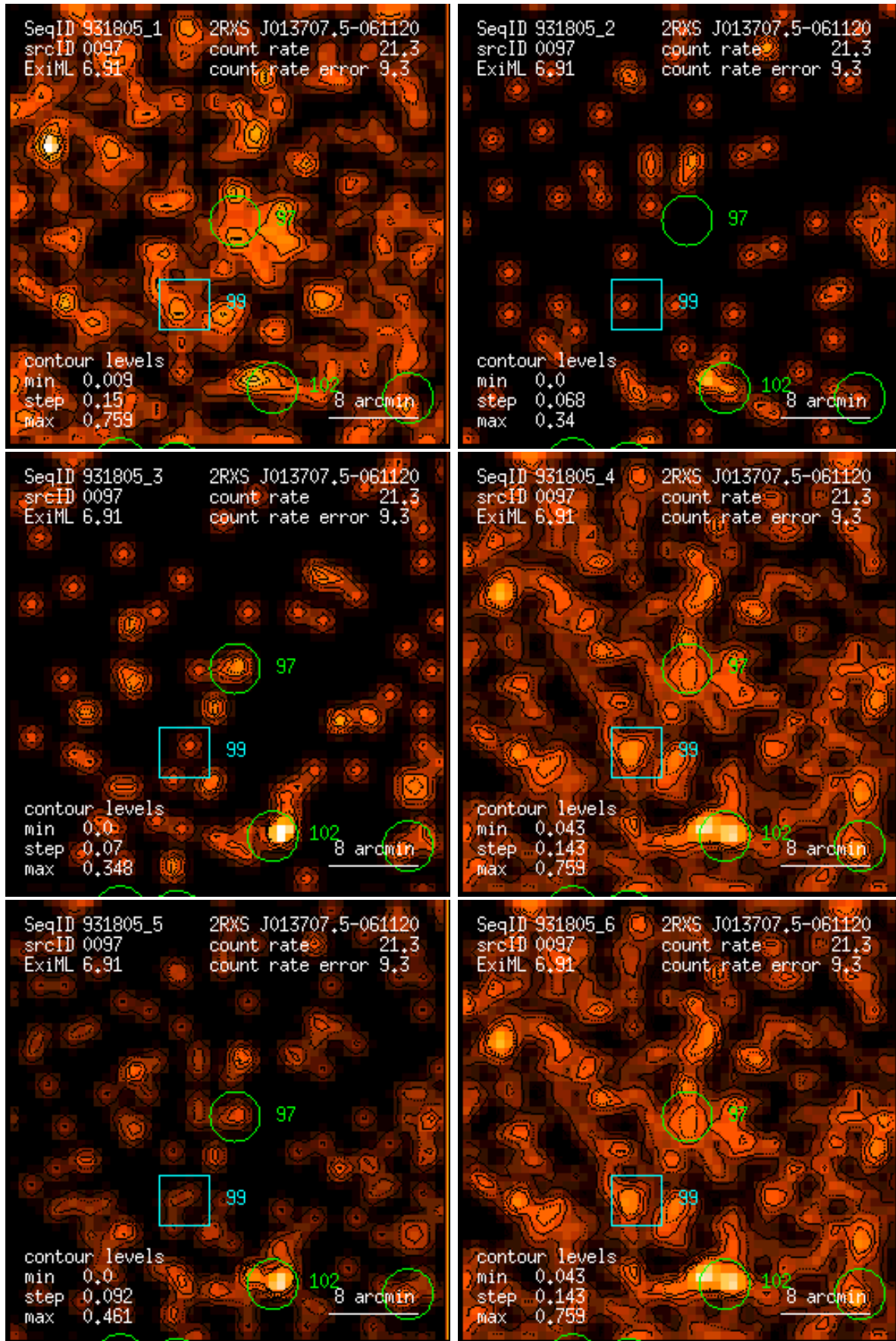
Figure 97: RASS 931805: detection 0097: band rate images, Gaussian filter: (1) PSPC channels 11 – 41, (2) 52 – 90, (3) 91 – 201, (4) 11 – 235, (5) 52 – 201, (6) 11 – 201. Broad band rates in counts/ks. Band rate contour levels in counts/ks/arcmin 2 .
