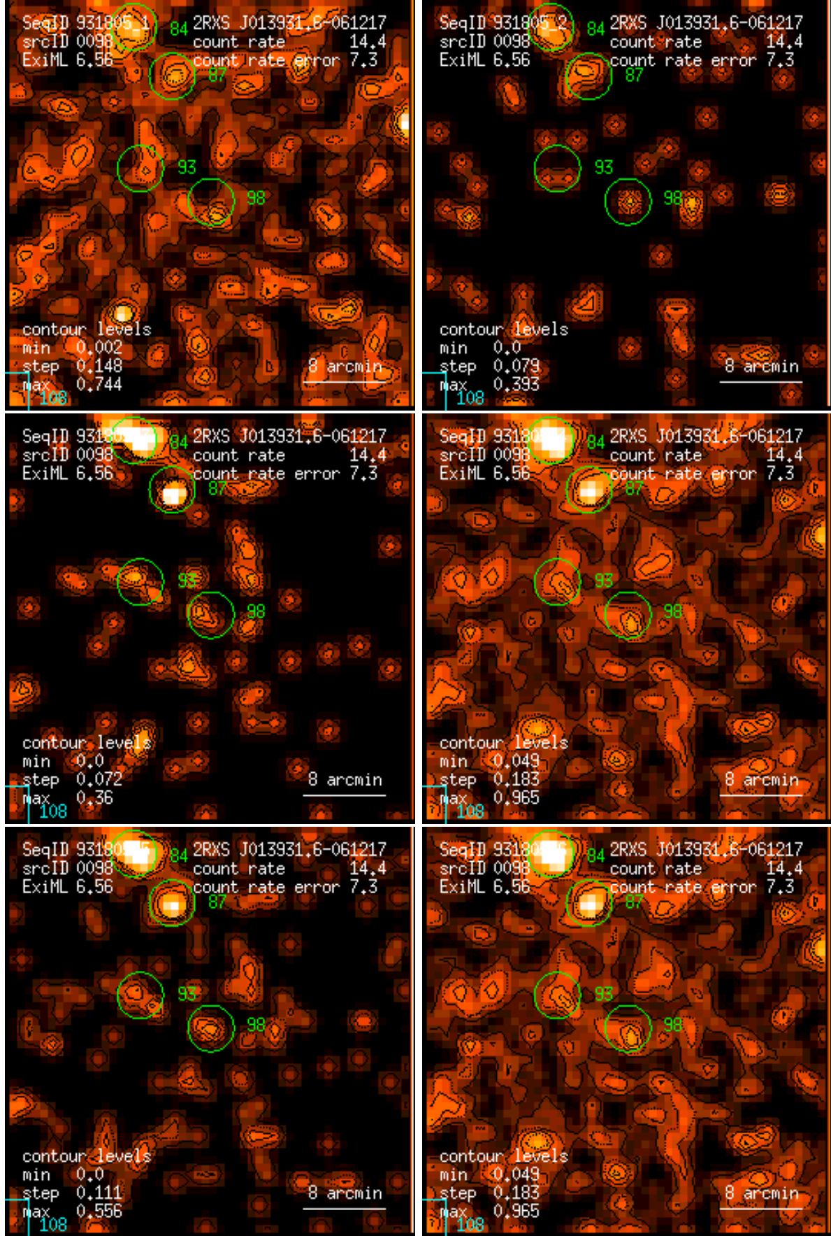
Figure 98: RASS 931805: detection 0098: band rate images, Gaussian filter: (1) PSPC channels 11 – 41, (2) 52 – 90, (3) 91 – 201, (4) 11 – 235, (5) 52 – 201, (6) 11 – 201. Broad band rates in counts/ks. Band rate contour levels in counts/ks/arcmin 2 .
