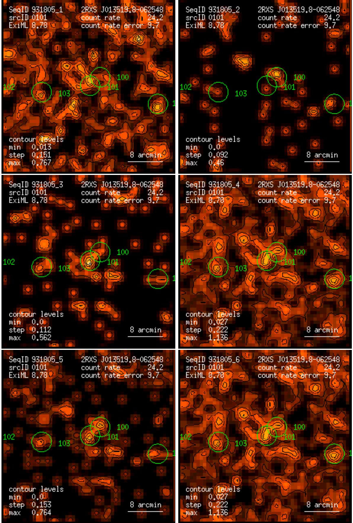
Figure 101: RASS 931805: detection 0101: band rate images, Gaussian filter: (1) PSPC channels 11 – 41, (2) 52 – 90, (3) 91 – 201, (4) 11 – 235, (5) 52 – 201, (6) 11 – 201. Broad band rates in counts/ks. Band rate contour levels in counts/ks/arcmin 2 .
