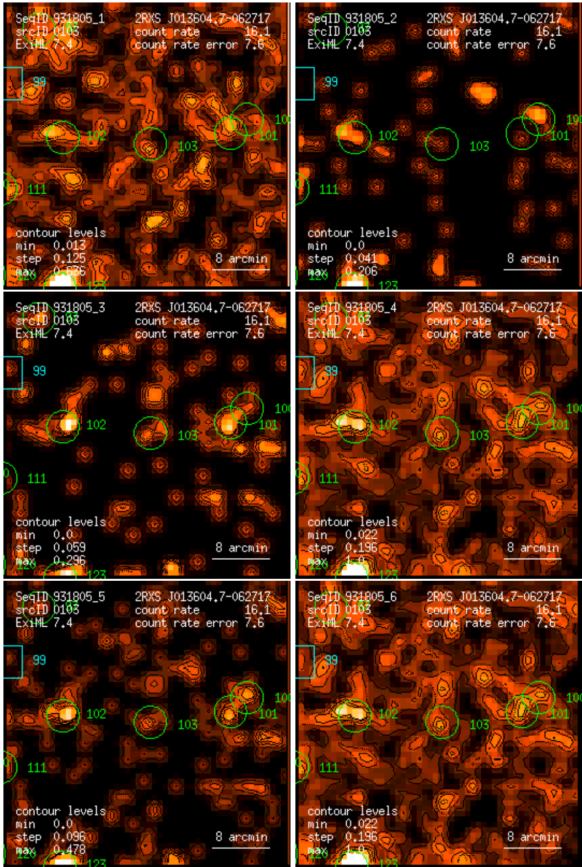
Figure 103: RASS 931805: detection 0103: band rate images, Gaussian filter: (1) PSPC channels 11 – 41, (2) 52 – 90, (3) 91 – 201, (4) 11 – 235, (5) 52 – 201, (6) 11 – 201. Broad band rates in counts/ks. Band rate contour levels in counts/ks/arcmin 2 .
