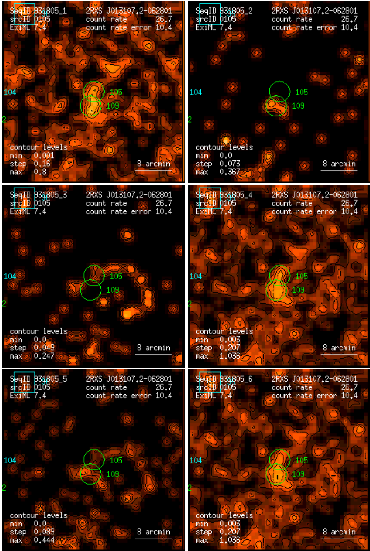
Figure 105: RASS 931805: detection 0105: band rate images, Gaussian filter: (1) PSPC channels 11 – 41, (2) 52 – 90, (3) 91 – 201, (4) 11 – 235, (5) 52 – 201, (6) 11 – 201. Broad band rates in counts/ks. Band rate contour levels in counts/ks/arcmin 2 .
