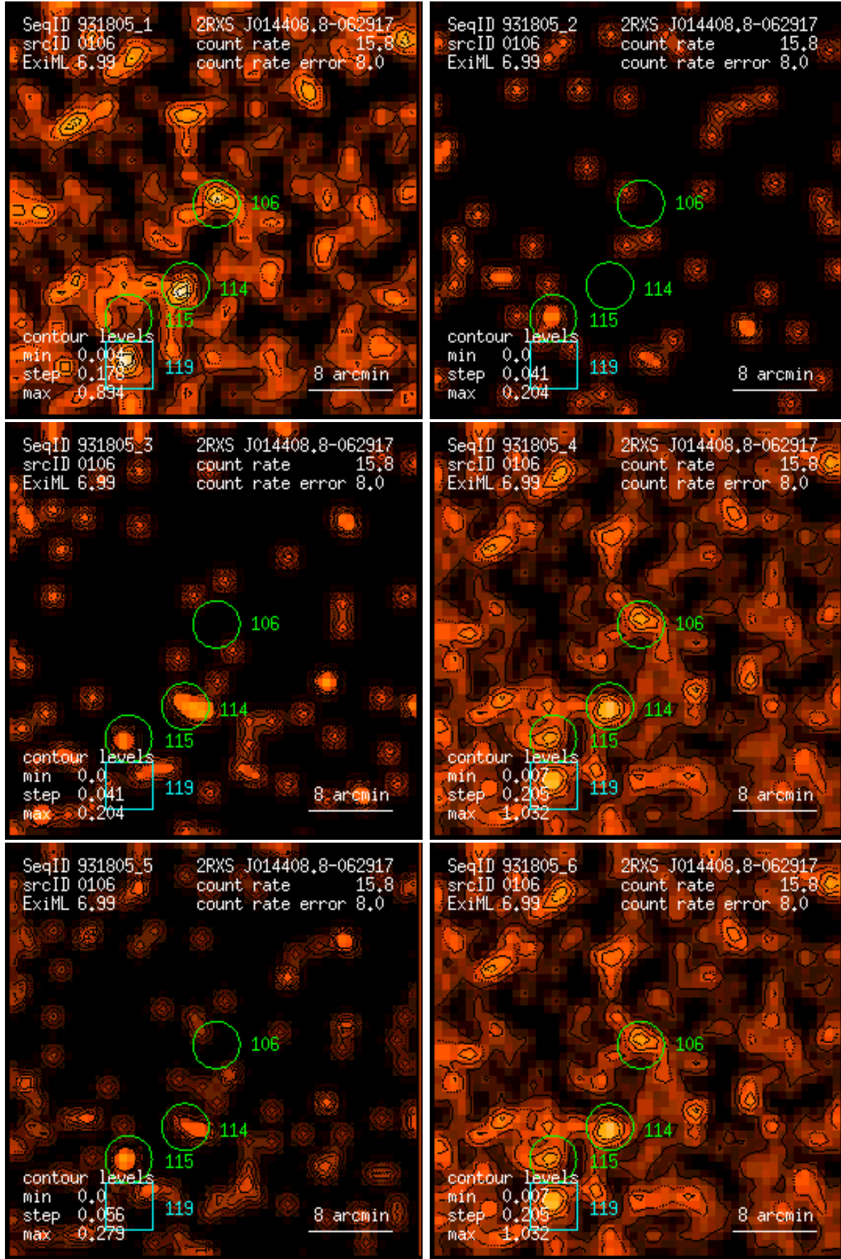
Figure 106: RASS 931805: detection 0106: band rate images, Gaussian filter: (1) PSPC channels 11 – 41, (2) 52 – 90, (3) 91 – 201, (4) 11 – 235, (5) 52 – 201, (6) 11 – 201. Broad band rates in counts/ks. Band rate contour levels in counts/ks/arcmin 2 .
