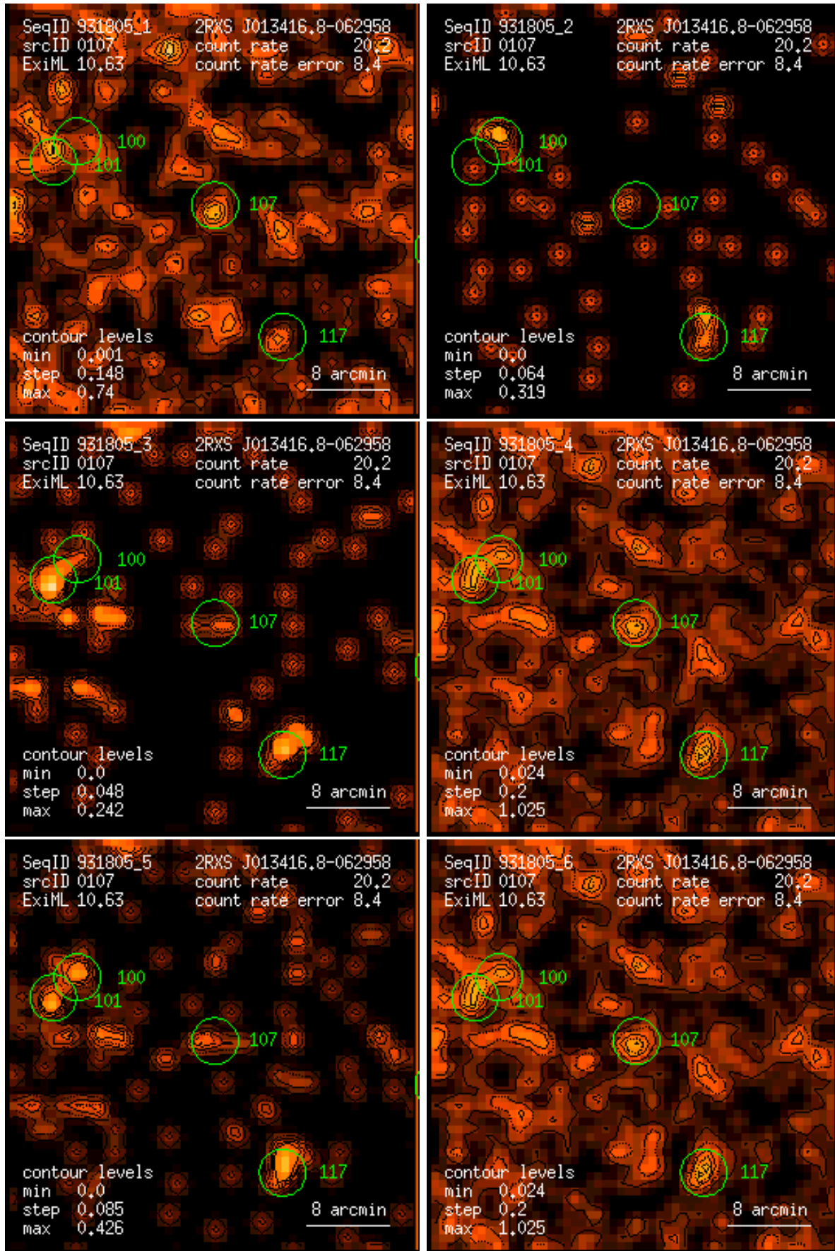
Figure 107: RASS 931805: detection 0107: band rate images, Gaussian filter: (1) PSPC channels 11 – 41, (2) 52 – 90, (3) 91 – 201, (4) 11 – 235, (5) 52 – 201, (6) 11 – 201. Broad band rates in counts/ks. Band rate contour levels in counts/ks/arcmin 2 .
